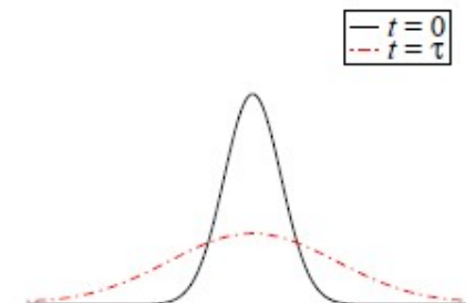
Fig. 10.8 Deterministic decay of an initial state. An initial condition with the same density will slowly decay to zero.
