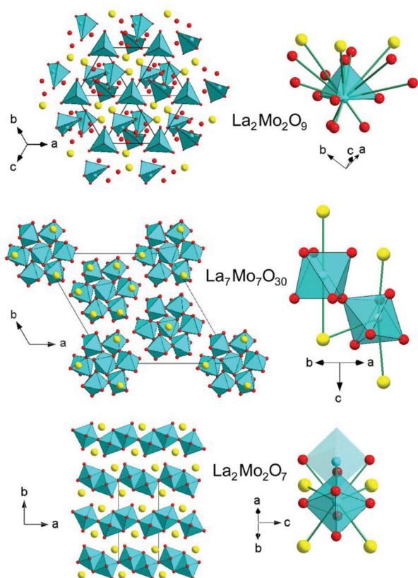
Fig. 2 Global configuration (left) and local arrangement around Mo (right) in the structures of crystallized \beta -La 2 Mo 2 O 9 (upper), La 7 Mo 7 O 30 (middle) and La 2 Mo 2 O 7 (lower). Mo coordination polyhedra are in blue as well as Mo ions, La 3+ ions are in yellow and O 2- ions in red. Note that Mo coordination polyhedra are isolated in La 2 Mo 2 O 9 , corner-sharing in La 7 Mo 7 O 30 , and edge-sharing in La 2 Mo 2 O 7 .
