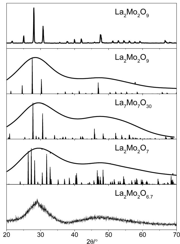
Fig. 3 XRD pattern of La 2 Mo 2 O 9 (top) and amorphous La 2 Mo 2 O 6.72 (bottom) with in between simulated XRD patterns of La 2 Mo 2 O 9 , La 7 Mo 7 O 30 and La 2 Mo 2 O 7 assuming large (narrow peaks) and very small crystallite sizes (broad envelopes) from PDF4+ database software. 28
