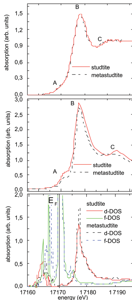
Fig. 4 Experimental (top) and calculated (middle) U L_3 -Edge HR-XANES spectra and calculated U d- and f-DOS (bottom) of studtite and metastudtite. The E_F line separates the occupied from the unoccupied DOS.
