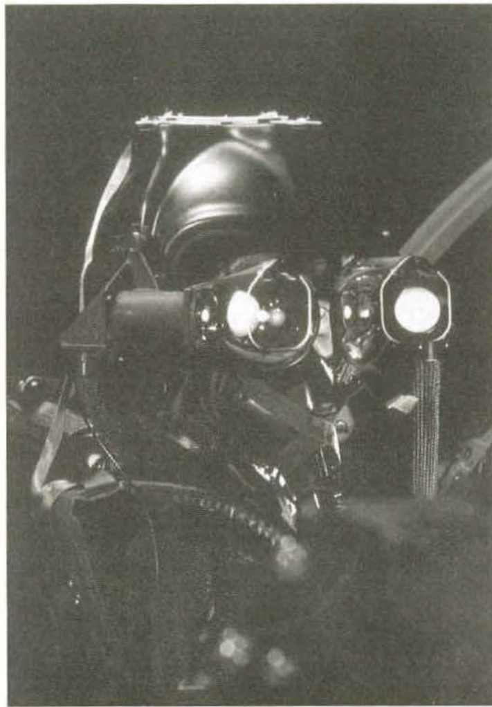
Figure 4.14 A pilot in the Tornado OBT wears a CAE helmet-mounted display. Military Systems & Trainings News , no. 1 (fall 1999/winter 2000): p. 7.
