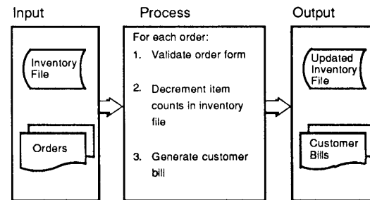
Fig 14 Input-Process-Output Chart
