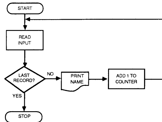
Fig 10 Flowchart
