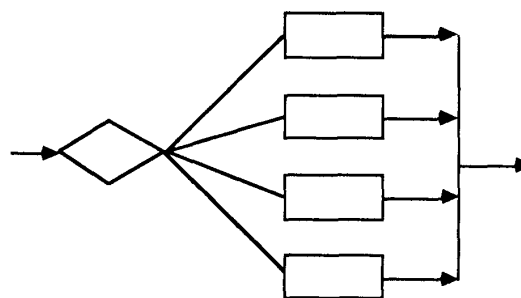
Fig 5 Case Construct
