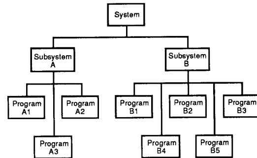
Fig 16 Structure Chart
