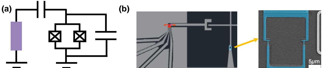
FIG. 1. Exemplary quantum circuit for analysis. (a) Circuit diagram. On the right side a SQUID (superconducting quantum interference device) composed of two Josephson junctions. This element is capacitively coupled to a resistive element on the left. (b) The actual on-chip circuit. The coupling capacitor is the fork-like structure in the middle, and the SQUID is zoomed out in blue on the right. The resistive element is contacted by four NIS tunnel junctions to control and measure temperature, on the left.
