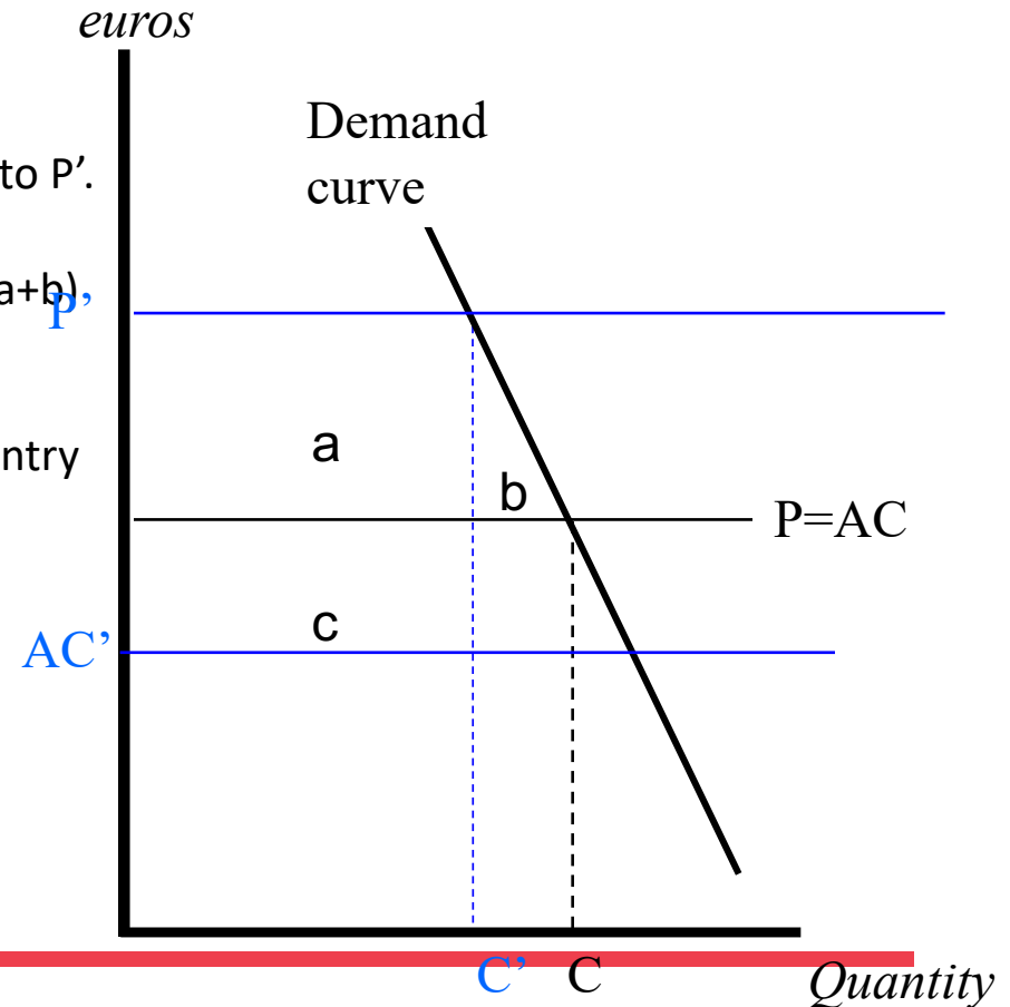
Williamson's diagram
