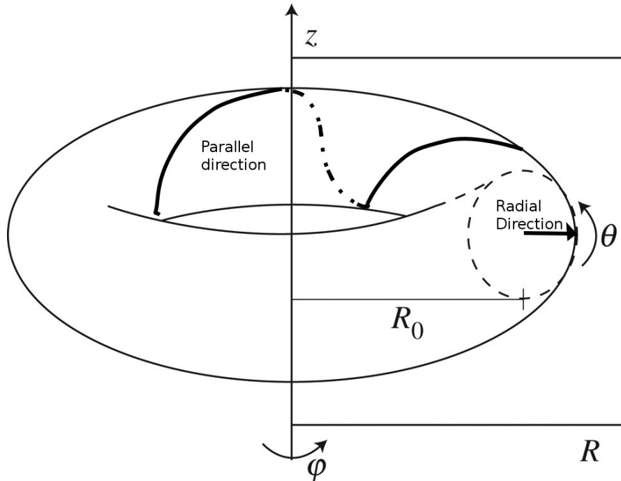
Figure 1: Schematic of tokamak coordinates used in exercise 1.
