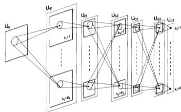
Fukushima's Neocognitron
