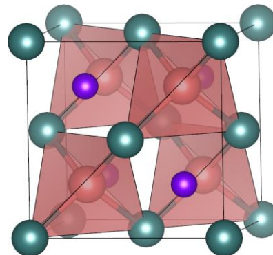
Another view, Si and Al 4-coordinated, Li^+ cations
