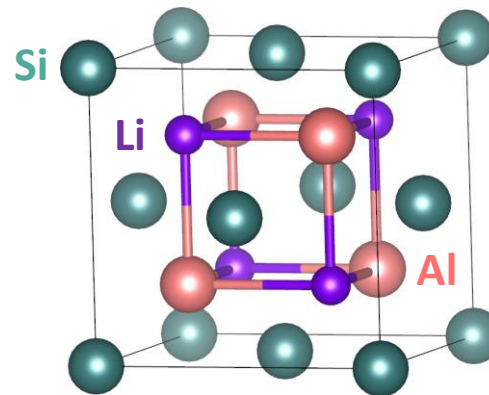
LiAlSi ( F-43m ) Si = X; Li = Y; Al = Z Semiconductor (8 valence e^- ) Can be considered as a Zintl phase! Li-Al drawn for clarity, not bonds
