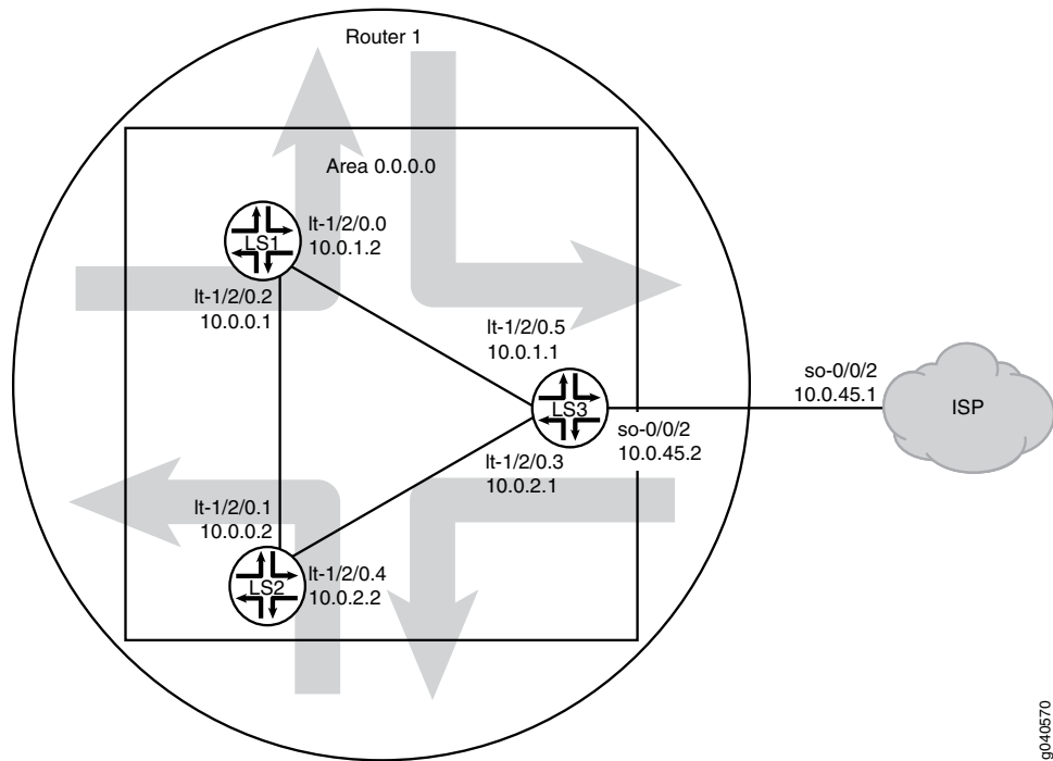
Figure 15: OSPF with a Conditional Default Route to an ISP
