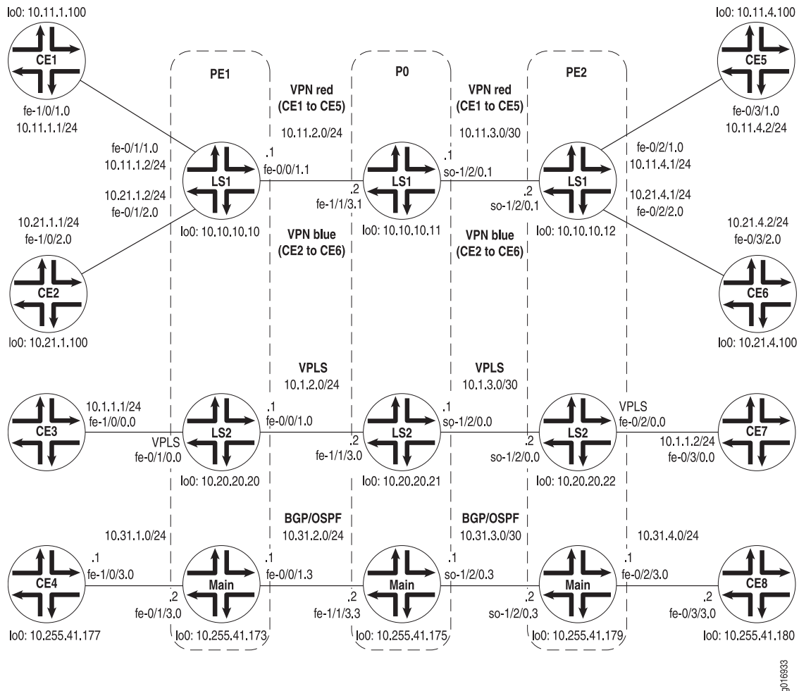
Figure 27: Provider Edge and Provider Logical System Topology Diagram
