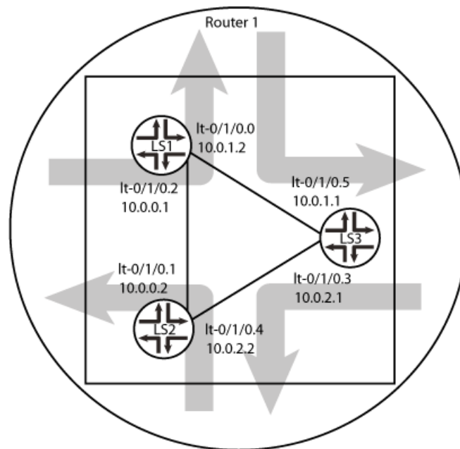
Figure 18: IS-IS on Logical Systems
