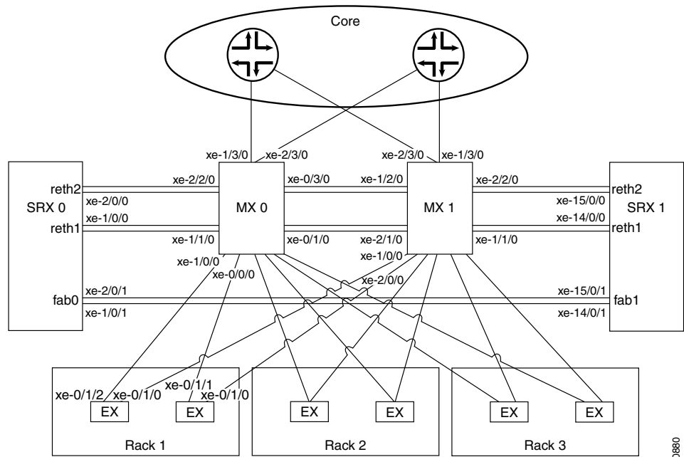
Figure 28: Virtualized Data Center Physical Topology
