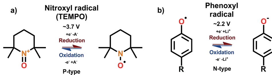
Fig. 13 Redox schemes for (a) nitroxyl radical TEMPO, and (b) phenoxy radicals. 68,70
