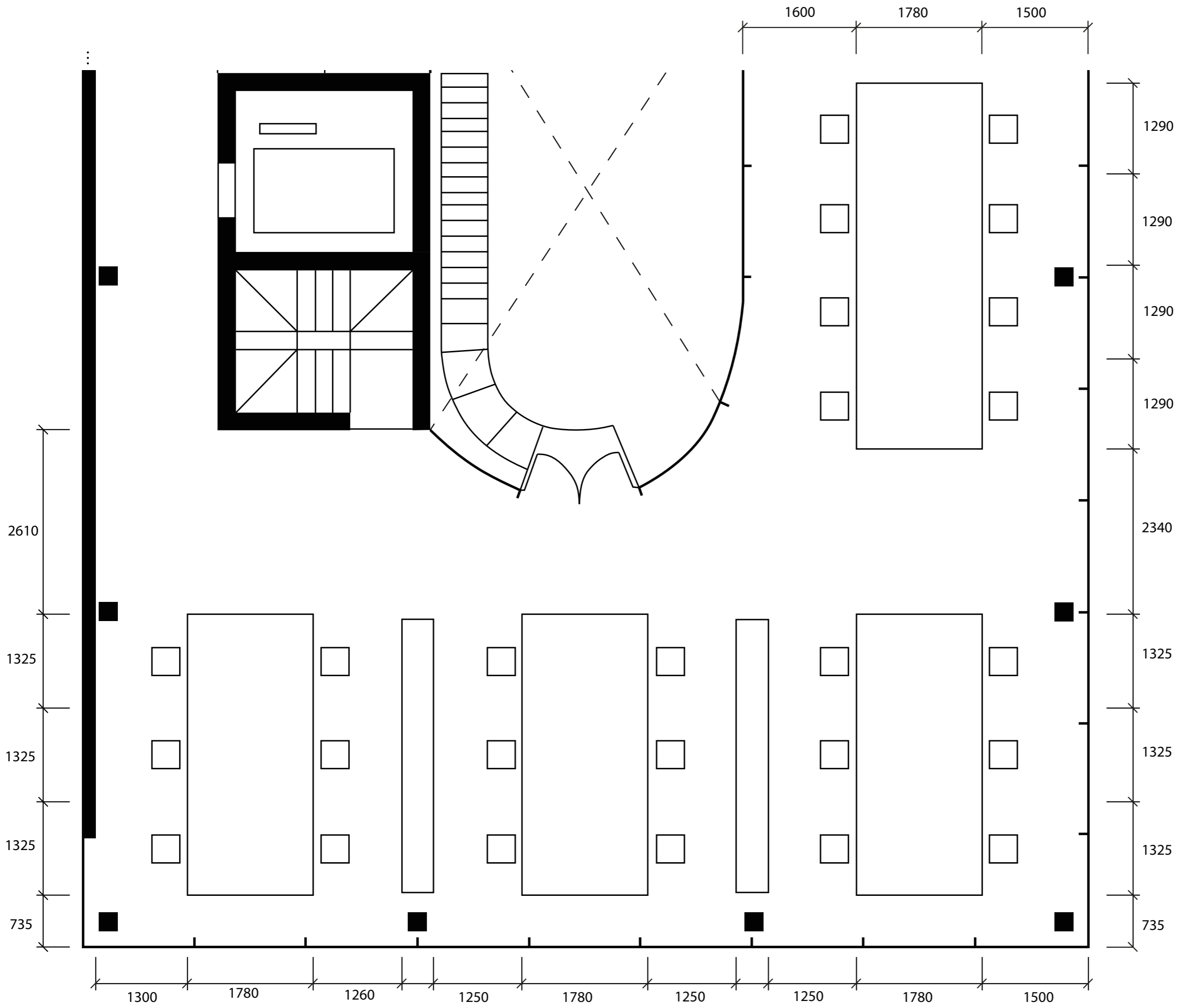
SHIBAURA HOUSE 3. KERROS 1:50
