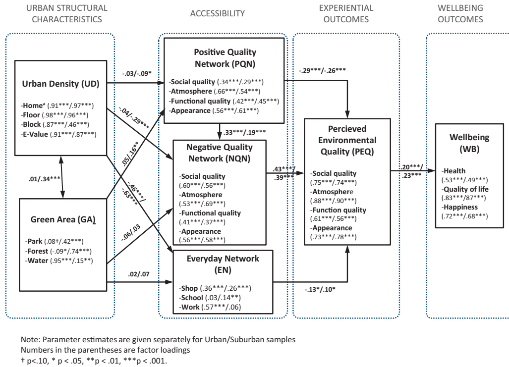
Figure 7. The model of analysis with the results of structural equation modeling.
