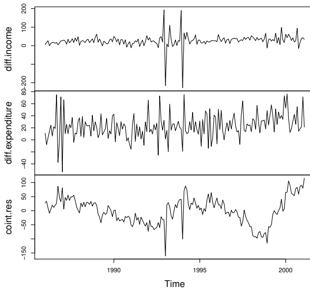
Figure 2: Time series used – first differences and cointegration residuals
