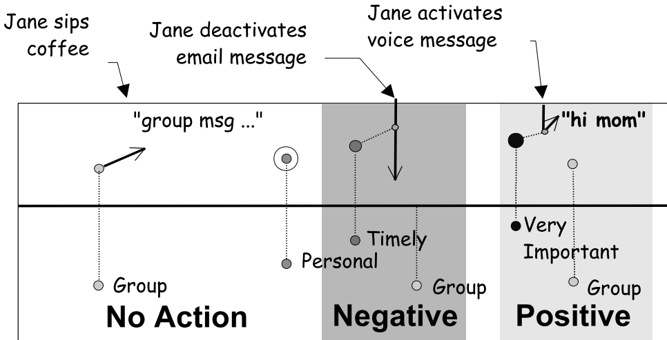
Fig. 9. Adaptation of notification weights based on Jane's actions while listening to messages.
