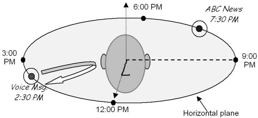
Fig. 4. Audio messages are positioned around the listener's head based on their time of arrival, providing a scalable presentation for browsing. Here, while the user is listening to an ABC (American Broadcasting Company) News broadcast in the background, an incoming voice message begins to play, gradually fading in and out of the listener's foreground. Spatialized audio allows the listener to segregate both messages, while focusing attention on the primary audio stream.
