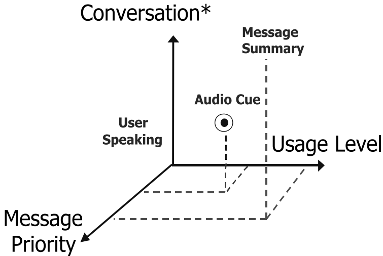
Fig. 8. The contextual notification model. Here only an auditory cue is presented for an incoming group message if the user is speaking and not actively using the device. However, a summary is spoken for urgent messages when the conversation level is lower. The conversation scale is shown inverted for simplicity.
