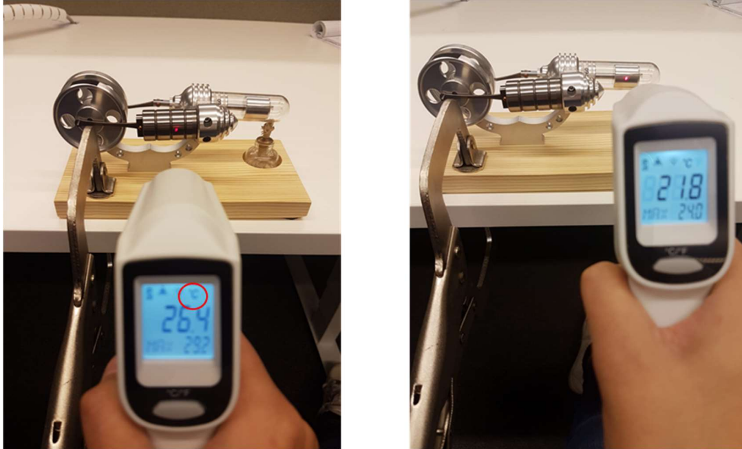
Figure 25 Temperature measurement settings.
