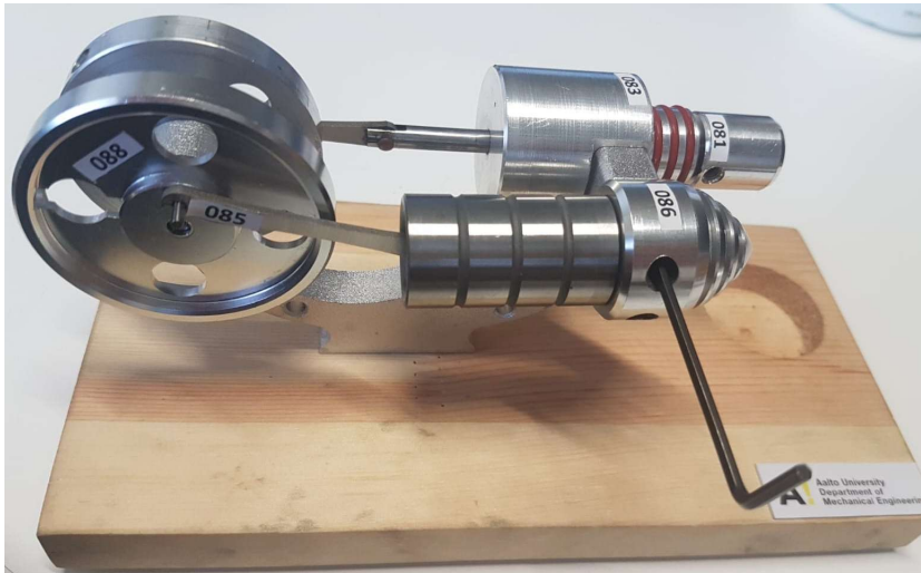
Figure 19 Flywheels, displacer piston, and power piston assembly.
