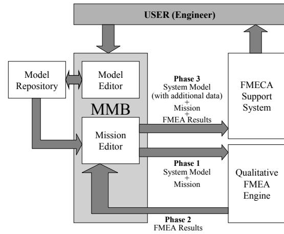
Figure 2. Software architecture
