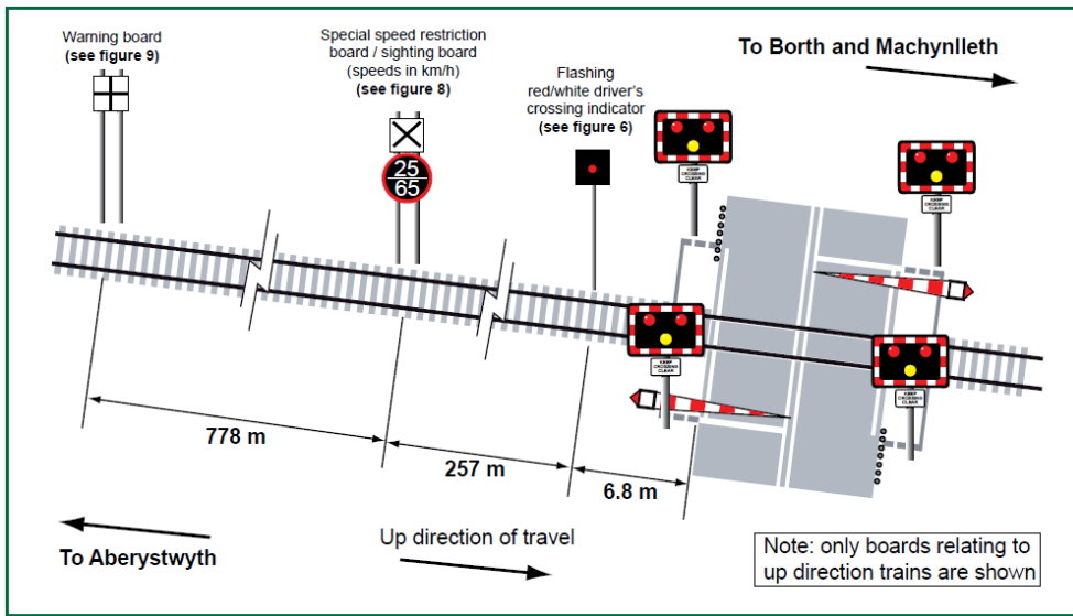
Figure 3. Schematic diagram of Llanbadarn ABCL.
