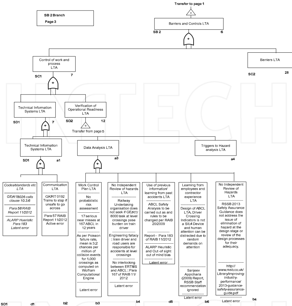
Figure 6. SIRI MORT SB2 Branch.
