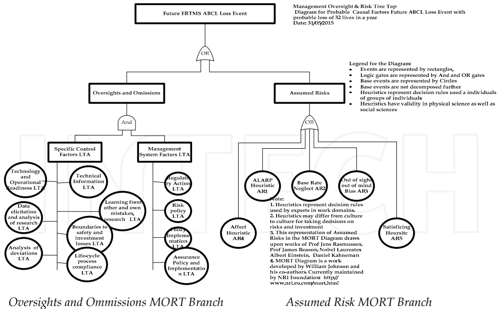
Figure 5. SIRI MORT Top Tree (Page 1)
