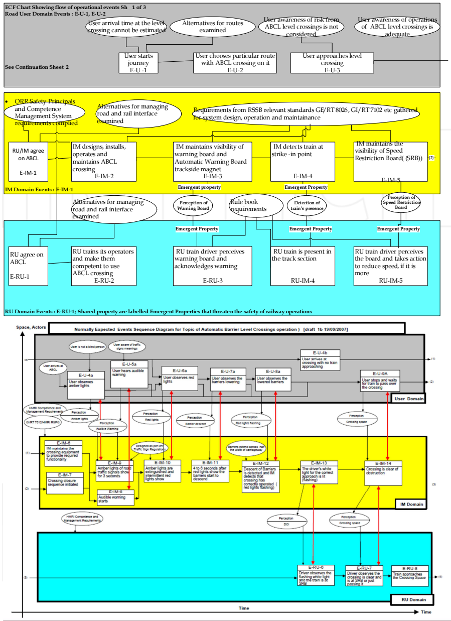
Figure 4. Representation of the concept of operations of ABCL Facility signalled by traditional lineside signalling
