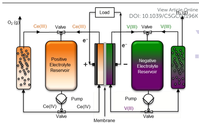
Figure 2. Dual-circuit redox flow battery architecture. The valves allow electrolyte to pass through the external reactors, where the electrolyte may be chemically discharged 'on demand' to produce hydrogen and oxygen on the negative and positive halves, respectively. 17
