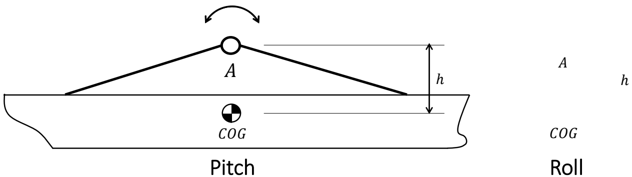
Figure 9-2 Sketch of a pendulum test
