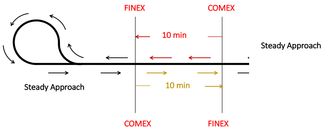
Figure 9-5 Trial trajectory of one double run (ITTC- recommended procedures and guidelines)
