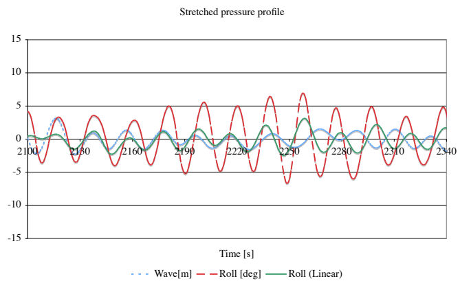
Fig. 5 Built-up of a resonant roll motion in irregular stern quartering waves simulated using stretched wave pressure model.
