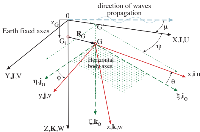
Figure 1. Co-ordinate systems used to describe ship motion (Matusiak, 2007)
