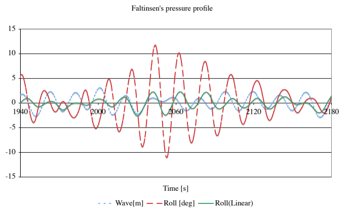
Fig. 4 Built-up of a resonant roll motion in irregular stern quartering waves simulated using the wave pressure model of Faltinsen.
