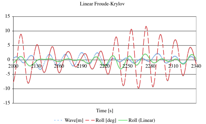
Fig. 3 Built-up of a resonant roll motion in irregular stern quartering waves simulated using a linear Froude-Krylov pressure model.
