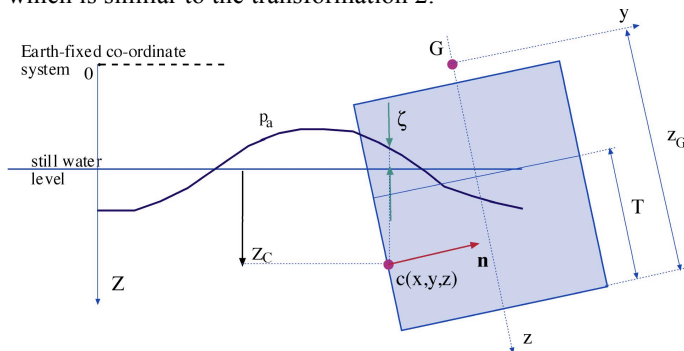
Figure 2. Evaluation of hydrostatic and Froude-Krylov pressure.
