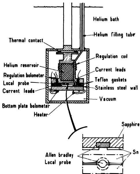
"HELIUM IN A SMALL BOX." Albert Libchaber's delicate experiment: Its heart was a carefully machined rectangular cell containing liquid helium; tiny sapphire "bolometers" measured the fluid's temperature. The tiny cell was embedded in a casing designed to shield it from the noise and vibration and to allow precise control of the heating.
