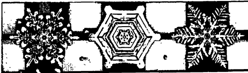
BALANCING STABILITY AND INSTABILITY. As a liquid crystallizes, it forms a growing tip (shown in a multiple-exposure photograph) with a boundary that becomes unstable and sends off side-branches ( left ). Computer simulations of the delicate thermodynamic processes mimic real snowflakes ( above ).
