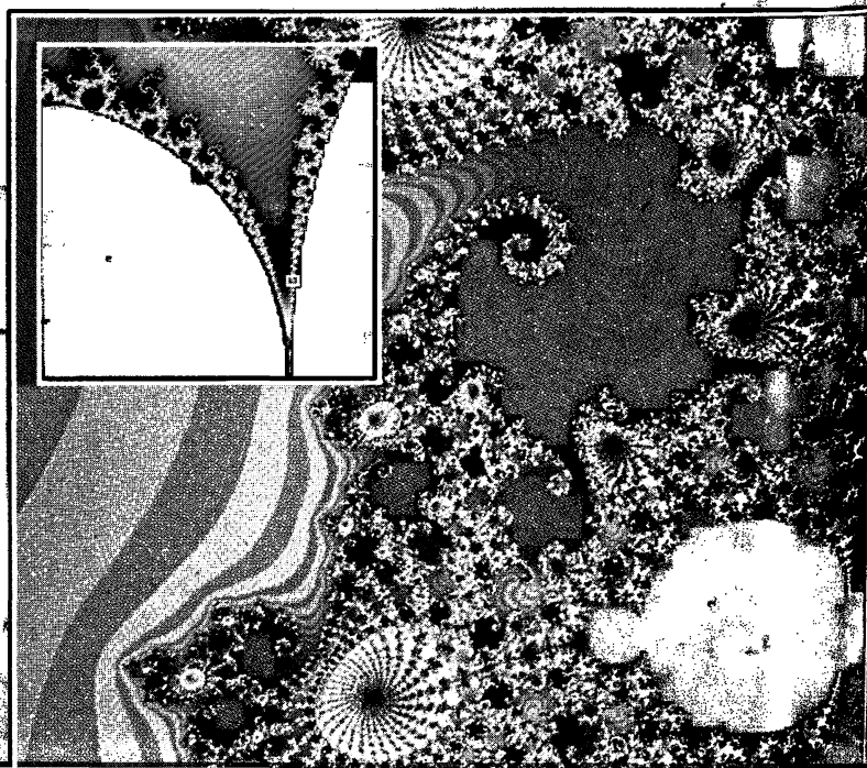
THE MANDELBROT SET —A voyage through finer and finer scales shows the increasing complexity of the set, with its seahorse tails and island molecules resembling the whole set. By the last frame, the level of magnification is about one million in each direction.
