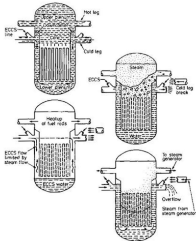
Phases of large-break LOCA.
