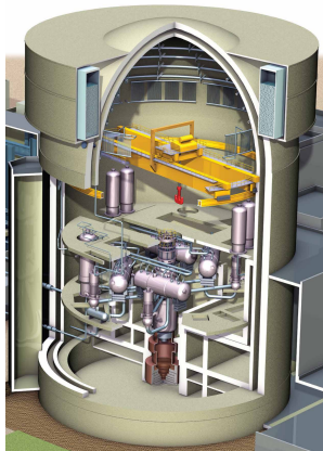
A reactor building and a primary circuit.
