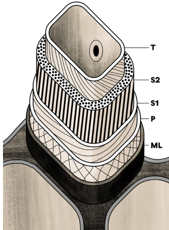
FIGURE 2 – Wood cell wall T: Inner layer S2: Middle layer S1: Outer layer P: Primary wall ML: Middle lamella
