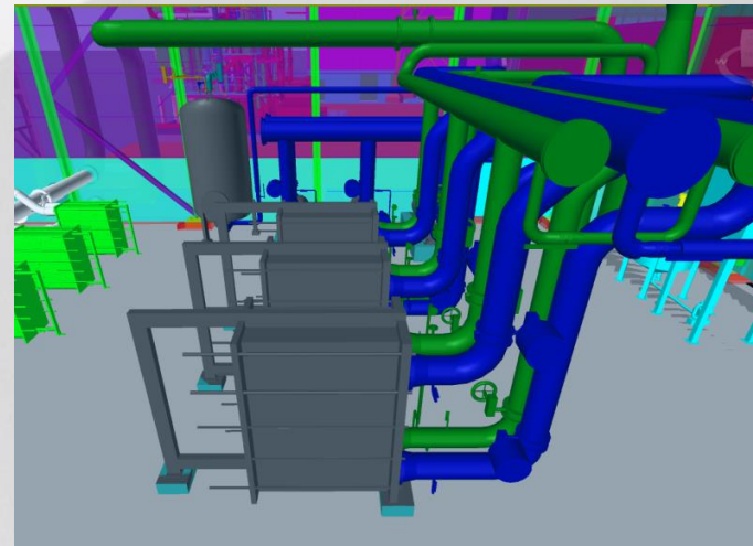
3D Piping design according to PI-diagram
