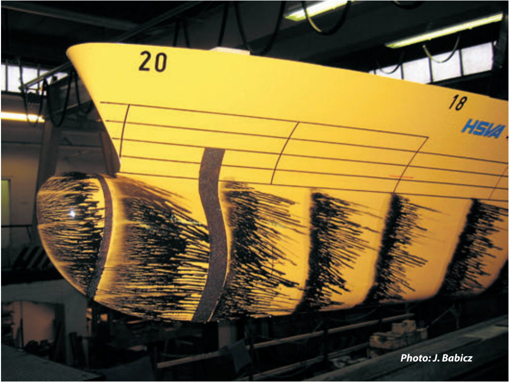
Model of container vessel VENUS tested at the Hamburg Ship Model Basin HSVA Hull shape designed by BOG-Projekt
