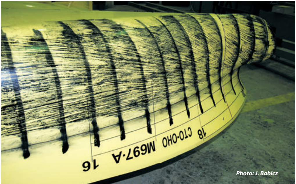
Model of MPV ARIADNA after paint test at the Gdańsk Ship Model Basin CTO S.A. Hull shape designed by BOG-Projekt
