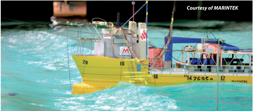
Seakeeping test
