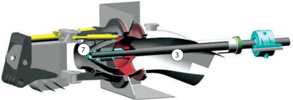
Waterjet with steering and reversing capability
