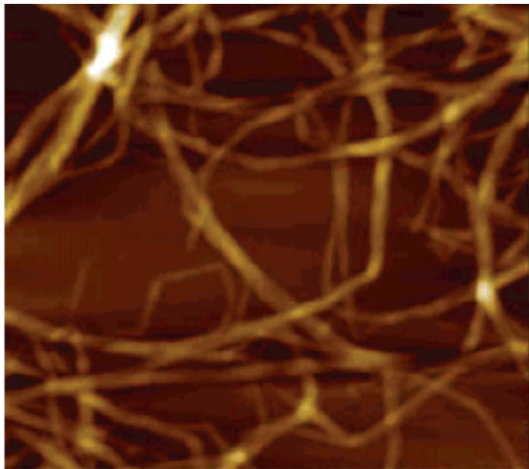
AFM image of cellulose nanofibres (CNF)
