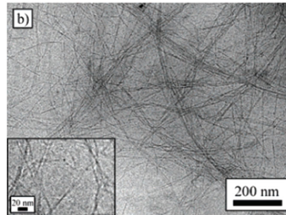
Cryo-TEM image of cellulose nanofibres (CNF)
