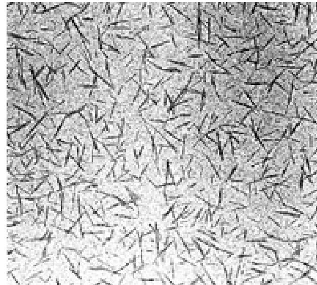
CNCs by TEM
