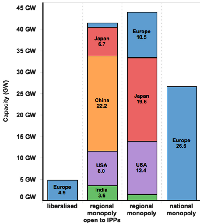
Fig. 2. Capacity (GW) of PHEs commissioned under different market structures.
