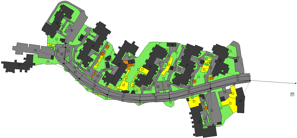
Figure 1. SWMM model view of Catchment 1.
