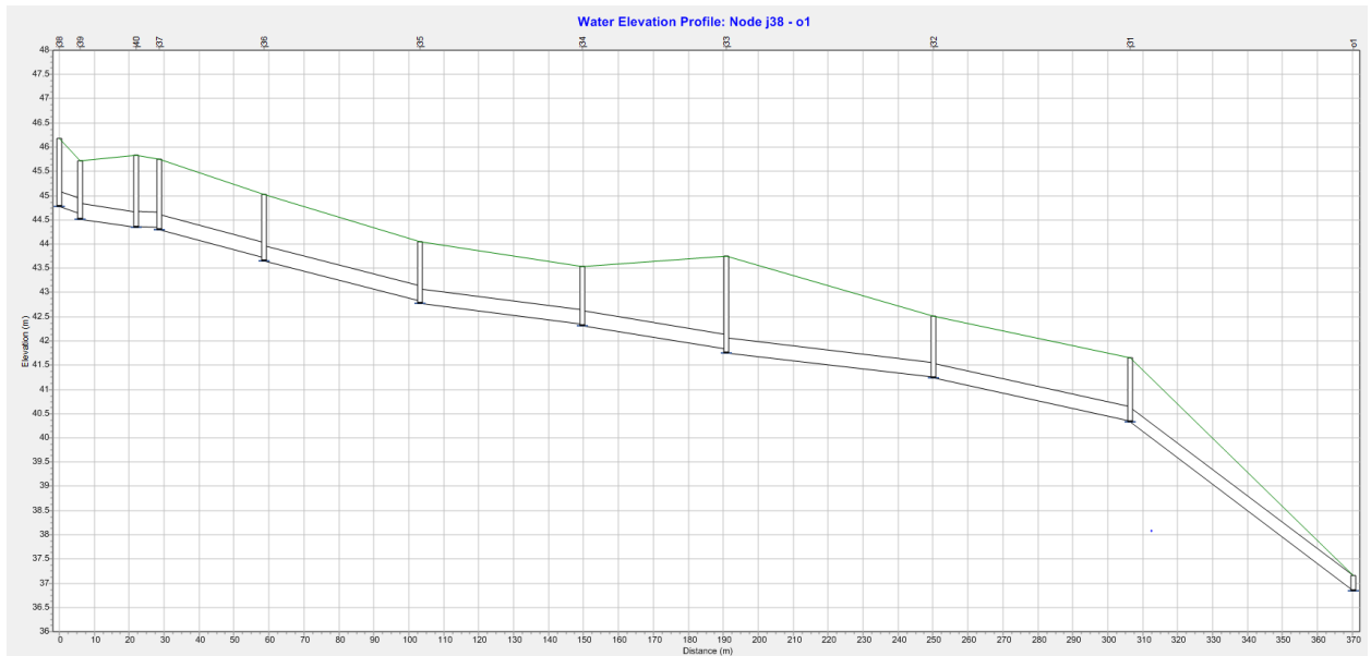
Figure 3. An elevation profile of the sewer network at Catchment 1.
