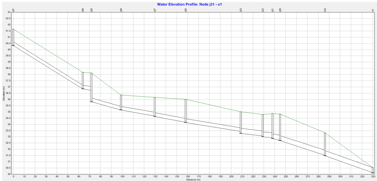
Figure 3. An elevation profile of the sewer network at Catchment 2.
