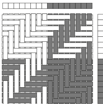
COLOUR AND WEAVE EFFECT
