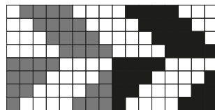
I / C 4:4 BROKEN TWILL
