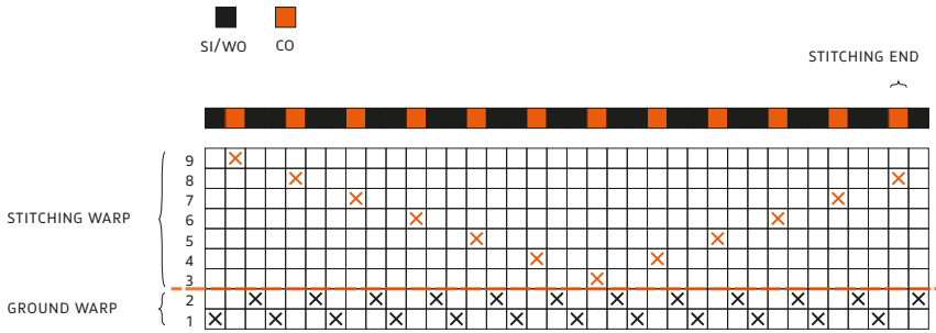
II / WADDING PICK STITCHING ON THE FACE
