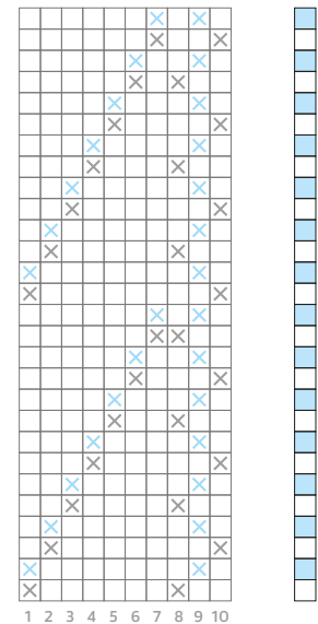
TIE-UP AND TREADLING
