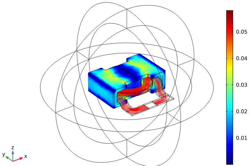
Streamline: Coil direction Volume: Magnetic flux density norm (T)
