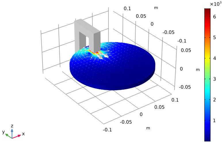
Figure 2: The eddy current magnitude and direction in the spinning disc of a magnetic brake.
