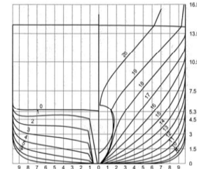
Stern Bow Body plan
