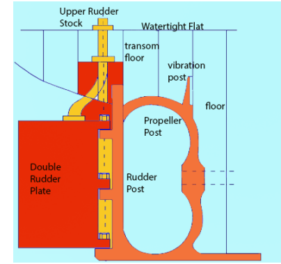
Unbalanced rudder
