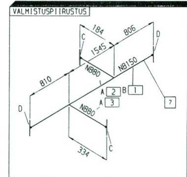
Production drawings
