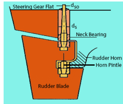
Semi-balanced rudder
