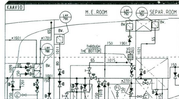
Installation drawings
