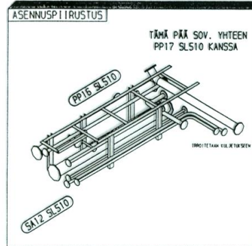
Installation drawings
