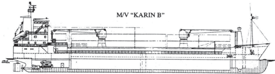
Fig. 3.42 Chemical Tanker, Shikoku Shipyard (Japan)
