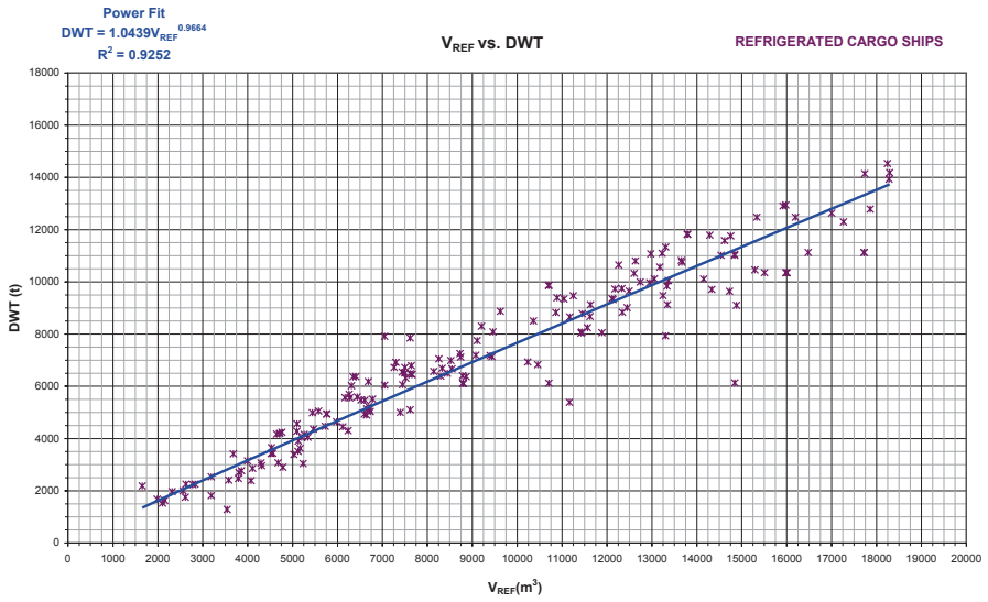
Fig. A.121 Regression analysis of the DWT [tons] versus the hold volume V_{REF} [m³] for reefer ships (Kalokairinos et al. 2000–2005)
