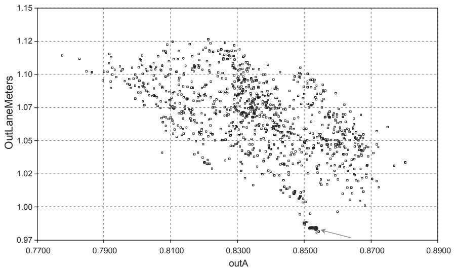
Fig. 1.38 Population of optimal design solutions (and Pareto front) of an RO-RO passenger ship with respect to the attained subdivision index A and the achieved length of vehicle lanes (Ship Design Laboratory—NTUA; Boulougouris 2003)
