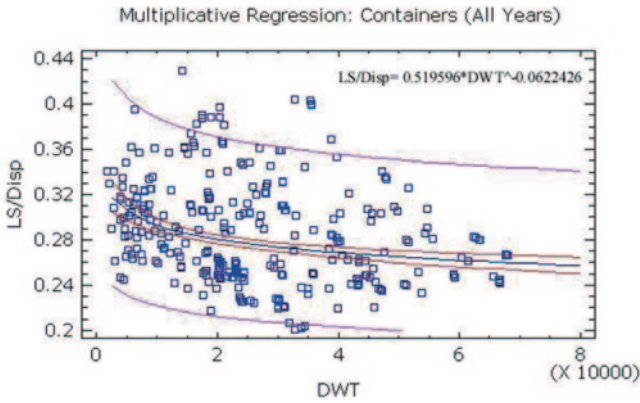
Fig. A.37 Regression analysis of ratio (LS/L) versus DWT [tons] for containerships* (Kalokairinos et al. 2000–2005)
