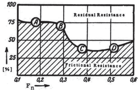
Fig. 2.9 Percentage shares of frictional resistance and residuary resistance for different ship types and characteristic Froude numbers by F. Horn (1930). A Slow cargo ship, B Transoceanic passenger ship, C Small passenger ship or cruiser, D Torpedo boat
