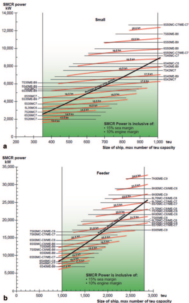
Fig. 2.60 Diagrams of installed propulsion power for containerhips versus DWT and speed V [knots]
