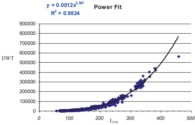
Fig. A.68 Regression analysis of DWT [tons] versus the length L_{OA} [m] for product carriers (Kalokairinos et al. 2000–2005)
