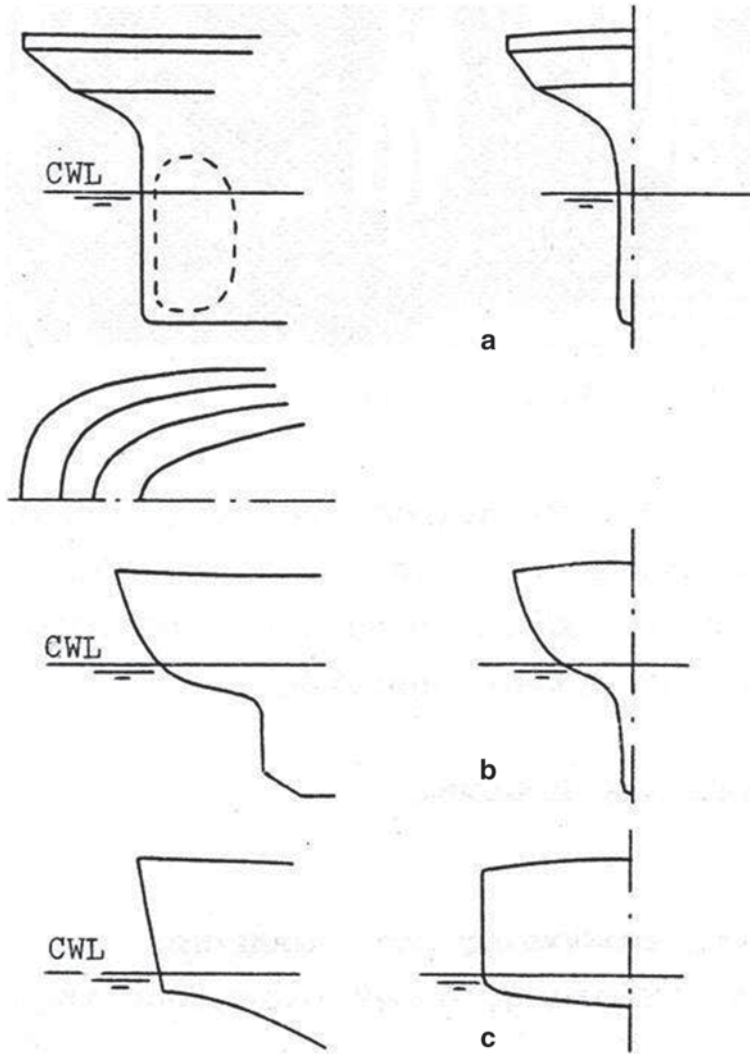
Fig. 3.61 Basic stern types
