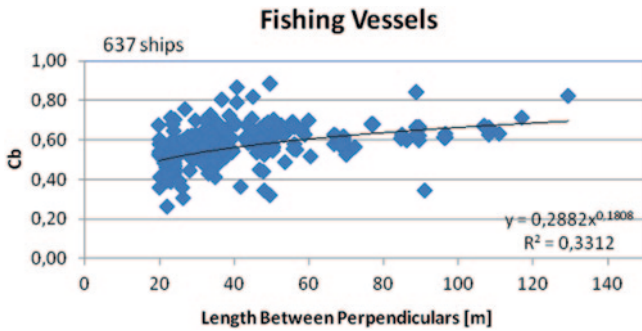
Fig. A.144 Regression analysis of the C_B versus the length between perpendiculars L_{BP} [m] for fishing vessels (IHS Fairplay 2011)
