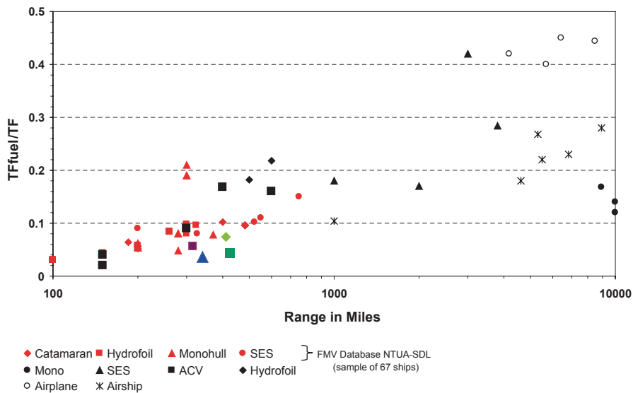
Fig. 1.8 Fuel transport factor ratio vs. range according to Kennell (1998) and NTUA-SDL. (Papanikolaou 2005)
