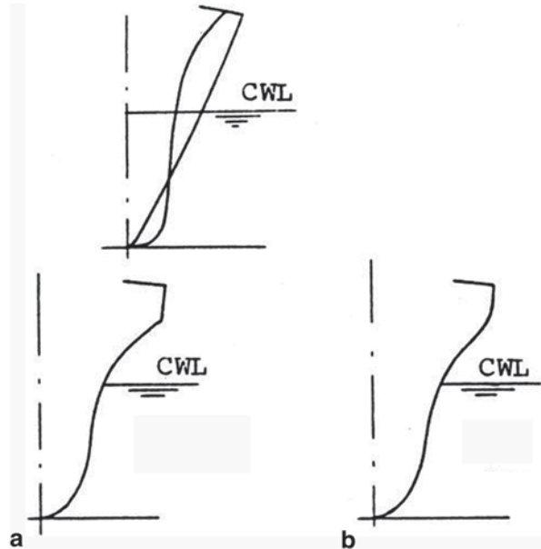
Fig. 3.27 Configuration of above waterline bow sections. a Above waterline section with hard chine. b Patented Deutsche Werft (“tulip” type) section
