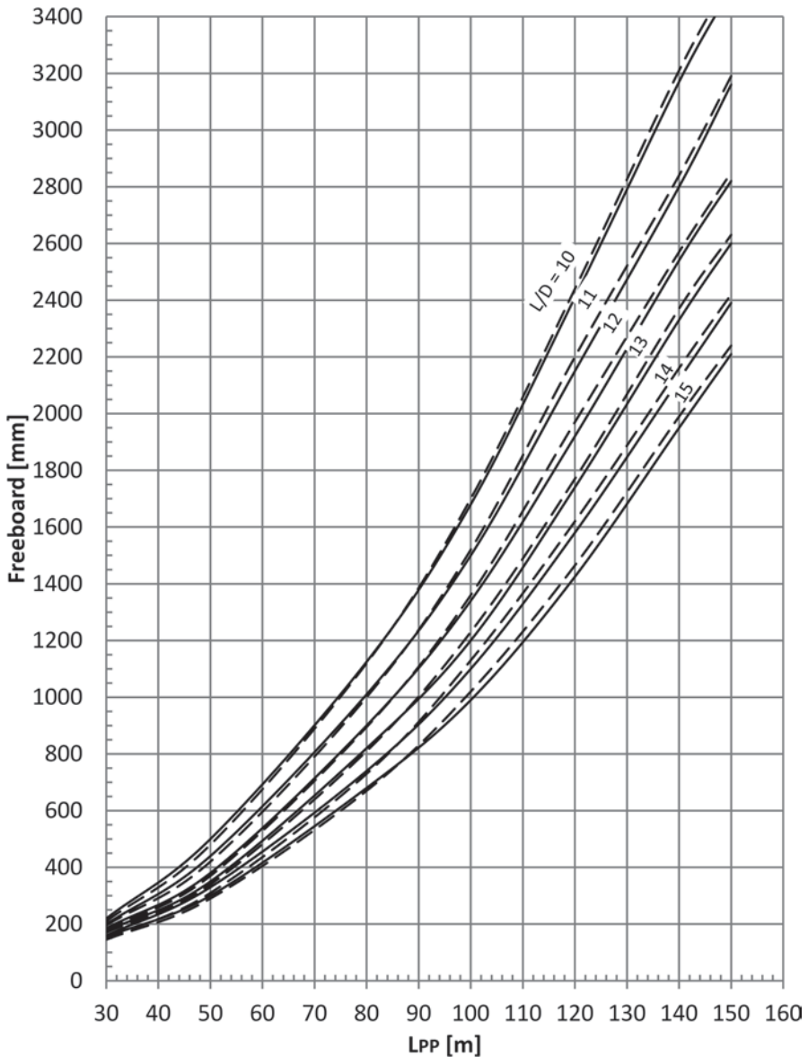
Fig. 2.107 Freeboard for dry cargo ships for l_s = 0.4 L_{pp} (———— ships with forecastle/poop, - - - - - ships with forecastle, poop, and superstructure amidships ( l_{Smidship} > 0.2 L_{pp} ))
