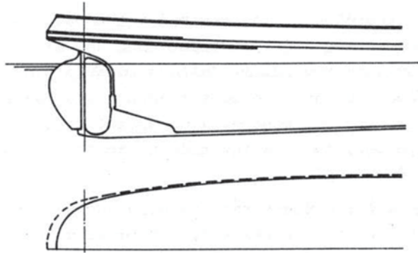
Fig. 3.63 Elliptical stern of tug boat
