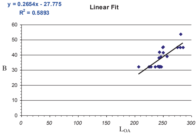
Fig. A.22 Regression analysis of beam B [m] versus length L_{OA} [m] for OBO carriers (Kalokairinos et al. 2000–2005)
