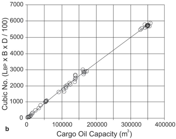
Fig. 2.24 Relations of L_{pp} and volumetric numeral L \times B \times D to the hold capacity for tankers. (Lamb 2003)
