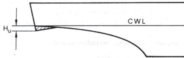
Fig. 3.67 Transom stern with wedge
