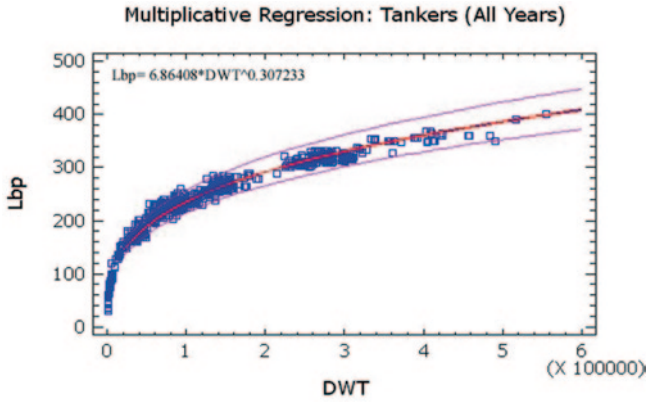
Fig. A.53 Regression analysis of length L_{BP} [m] versus DWT [tons] for tankers* (Kalokairinos et al. 2000–2005)
