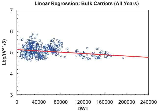
Fig. A.11 Regression analysis of slenderness ratio ( L/\nabla^{1/3} ) versus DWT [tons] for bulk carriers (Kalokairinos et al. 2000–2005)
