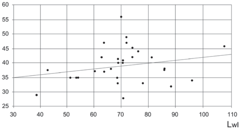
Fig. A.115 Regression analysis of the service speed V_s [knots] versus the length L_{wl} [m] for catamaran ferries according to Kristensen (2000) in Friis et al. (2002)
