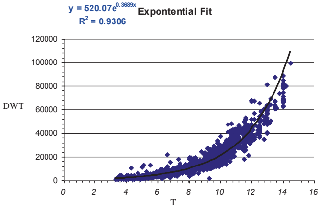
Fig. A.45 Regression analysis of DWT [tons] versus draft T [m] for containerships (Kalokairinos et al. 2000–2005)
