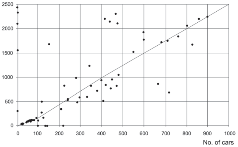
Fig. A.103 Regression analysis of the vehicles' lane length [m] versus the number of vehicles for RoPAX ships according to Kristensen (2000) in Friis et al. (2002)
