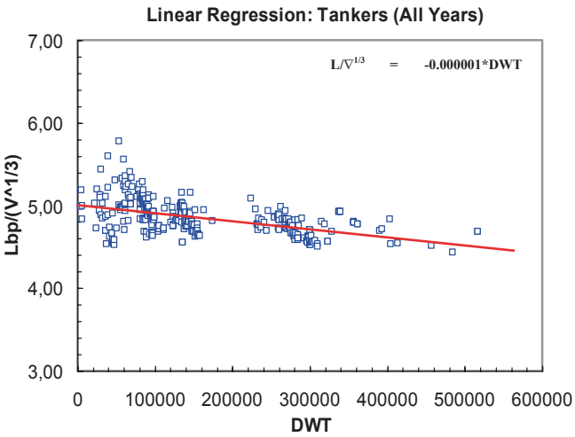
Fig. A.60 Regression analysis of slenderness ratio ( L/V^{1/3} ) versus DWT [tons] for tankers (Kalokairinos et al. 2000–2005)
