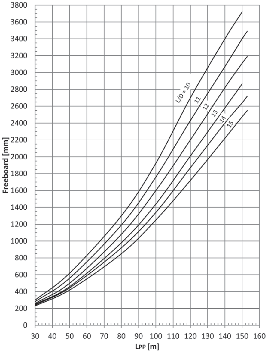
Fig. 2.104 Freeboard of dry cargo ships for l_s = 0.1 L_{pp}
