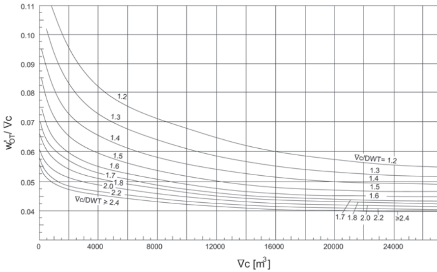
Fig. 2.79 Weight of outfitting versus the hold volume c and the ratio c/DWT for dry cargo ships according to Henschke (1964)
