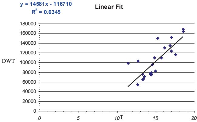
Fig. A.27 Regression analysis of DWT [tons] versus draft T [m] for OBO carriers (Kalokairinos et al. 2000–2005)
