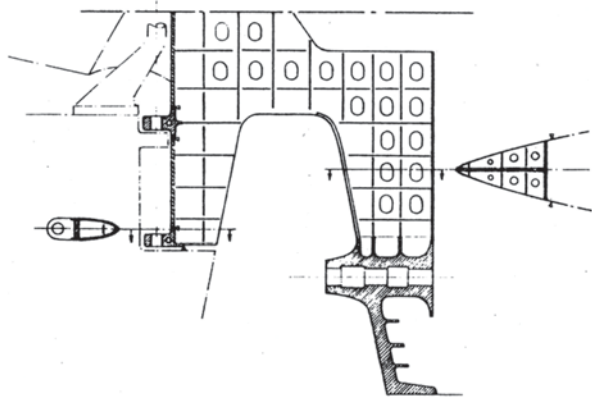
Fig. 5.48 Example of stern construction for semi-balanced, half-hanging rudder
