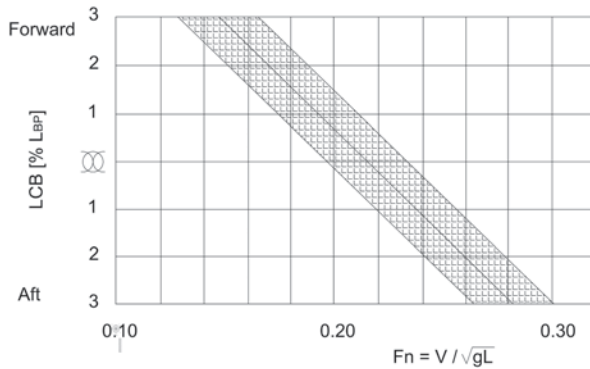
Fig. 3.5 Approximate optimal longitudinal position of center of buoyancy vs. Froude number according to Gulddammer-Harvard (1974)—Hull form series FORMDATA (Friis et al. 2002)
