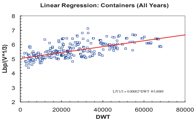
Fig. A.39 Regression analysis of slenderness ratio ( L/V^{1/3} ) versus DWT [tons] for containerships (Kalokairinos et al. 2000–2005)
