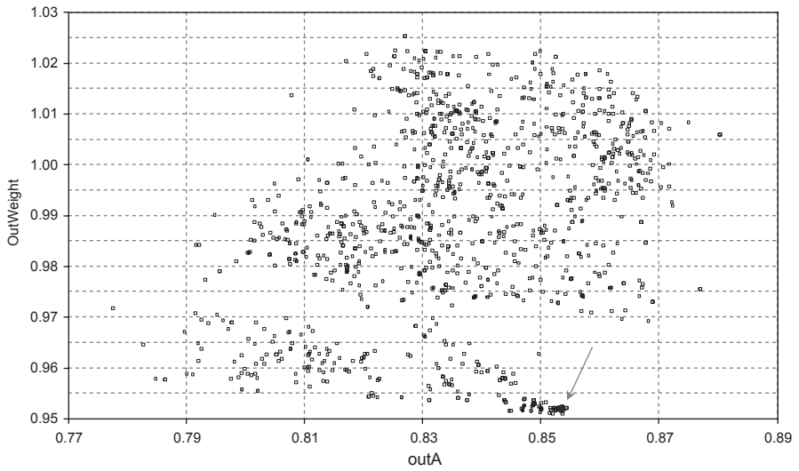
Fig. 1.39 Population of optimal design solutions (and Pareto front) of an RO-RO passenger ship with respect to the attained subdivision index A and a ship’s structural weight (Ship Design Laboratory—NTUA; Boulougouris 2003)
