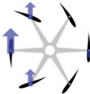
Fig. 5.30 Operational principle of Voith–Schneider Propeller
