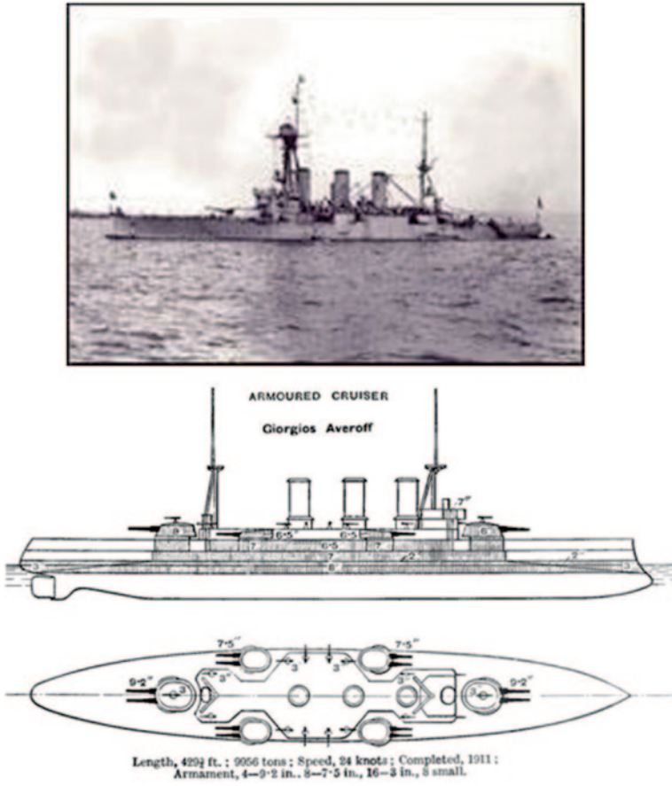
Fig. 3.32 WWI Greek battleship “Georgios Averof” (1910), L_{BP}=140.5 m, B=21 m, T=7.5 m, \Delta=10,118 t, P_S=19,000 HP, V=23.0 kn
