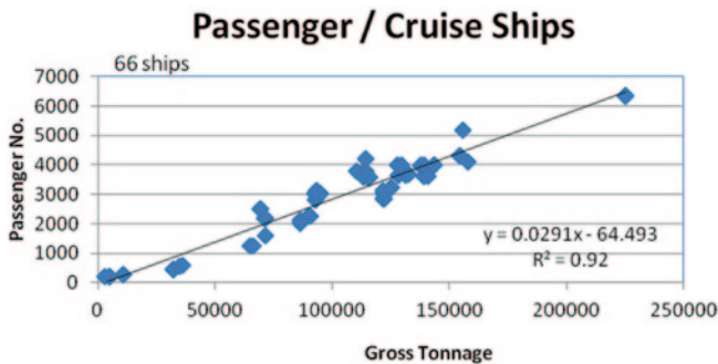
Fig. A.130 Regression analysis of the no. of passengers versus GT for cruise ships
