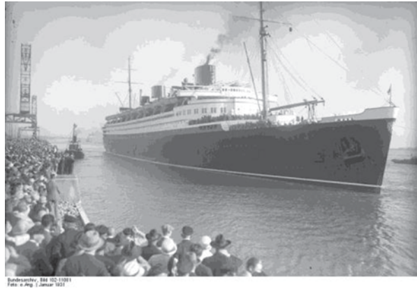
Fig. 3.31 German passenger ocean liner “Bremen” (1929), L=270.7 m, Displacement=51,860 t, Tonnage: 51,656 GRT, Shaft Horsepower=96,000 HP, V=28.5 kn (average speed, “blue ribbon” winner for crossing the Atlantic in year 1929)
