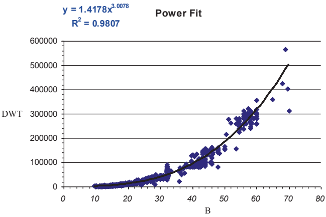
Fig. A.69 Regression analysis of DWT [tons] versus beam B [m] for product carriers (Kalokairinos et al. 2000–2005)
