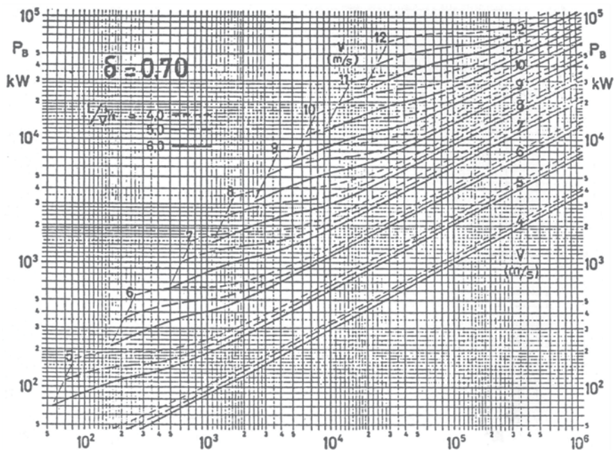
Fig. 2.64 Diagrams of installed propulsion power [kW] versus the displacement \Delta [tons], velocity V [m/s] and slenderness ratio L/V^{1/3} , C_B=0.70 acc. to Harvald
