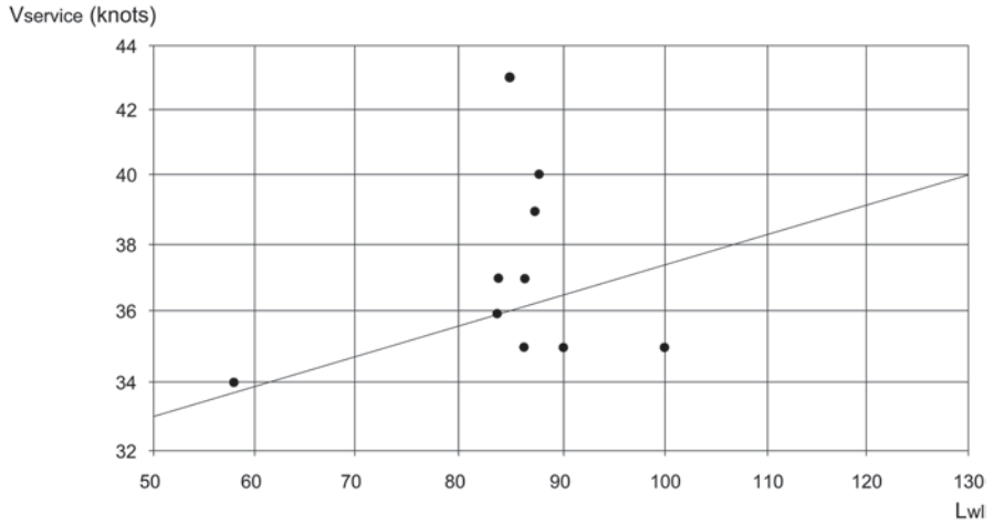
Fig. A.111 Regression analysis of the service speed V_s [knots] versus the length L_{wl} [m] for fast single-hull ferries according to Kristensen (2000) in Friis et al. (2002)
