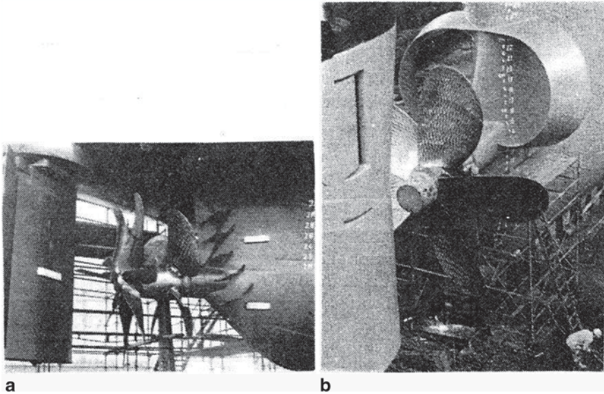
Fig. 3.25 Smoothing of flow to the propeller. a Propeller/stern fins and Grim's "vane wheel" behind the propeller. b Semi-duct according to Schneekluth (likewise the Becker-Mewis duct with integrated fin system within the duct)
