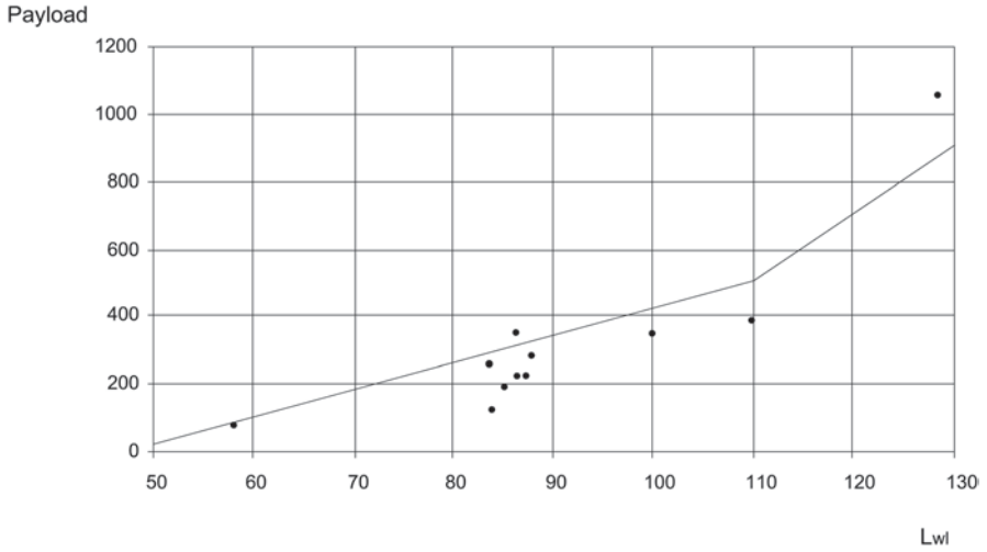
Fig. A.107 Regression analysis of the payload [tons] versus the length L_{wl} [m] for fast single-hull ferries according to Kristensen (2000) in Friis et al. (2002)
