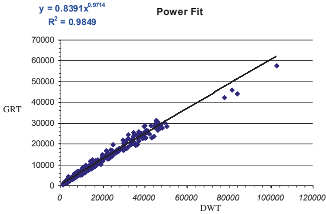
Fig. A.78 Regression analysis of GRT [RT] versus DWT [tons] for chemical carriers (Kalokairinos et al. 2000–2005)
