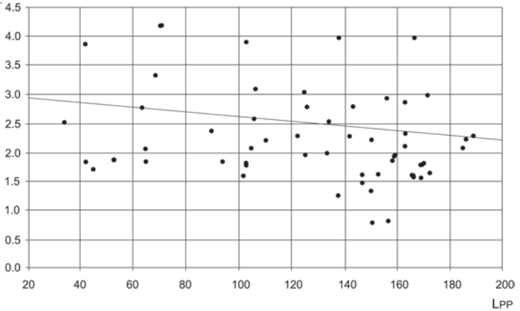
Fig. A.104 Regression analysis of the ratio of 60% of DWT [tons] to the vehicle lane length [m] versus the length L [m] for RoPAX ships according to Kristensen (2000) in Friis et al. (2002)
