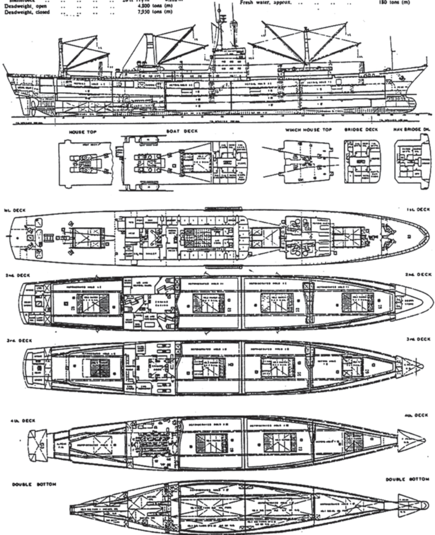
Fig. 4.13 General arrangement of reefer ship "Polar Ecuador," DWT=4800/7950 t
