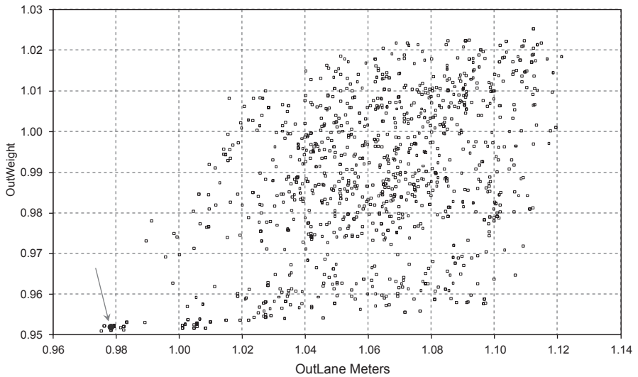
Fig. 1.40 Population of optimal design solutions (and Pareto front) of an RO-RO passenger ship with respect to the achieved length of vehicle lanes versus a ship’s structural weight (Ship Design Laboratory—NTUA; Boulougouris 2003)
