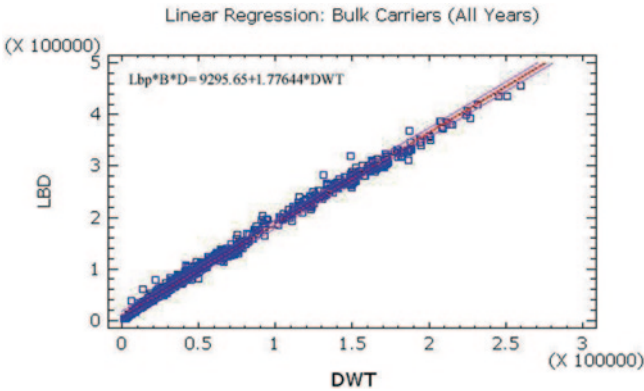
Fig. A.7 Regression analysis of the product (L \times B \times D) [m 3 ] versus DWT [tons] for bulk carriers* (Kalokairinos et al. 2000–2005)
