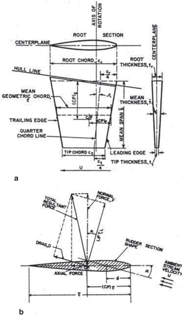
Fig. 5.34 a Typical dimensions of a rudder b Components of hydrodynamic rudder forces (Lewis 1988)
