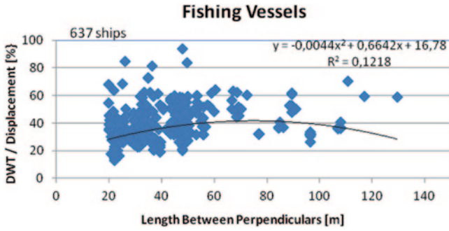
Fig. A.143 Regression analysis of the % DWT/Displacement ratio versus the length between perpendiculars L_{BP} [m] for fishing vessels (IHS Fairplay 2011)
