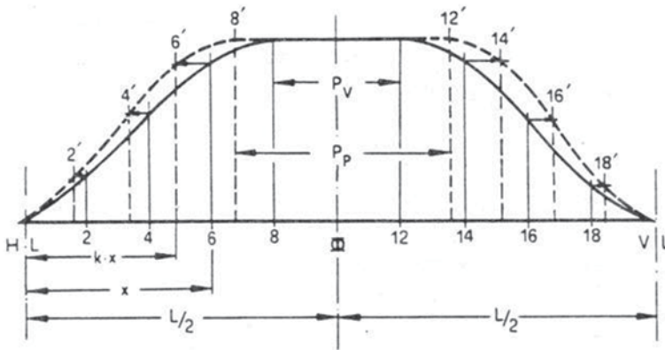
Fig. 4.10 Variation of section spacing with the change of the length of parallel body \delta L_p , where P_V \cong (L_p)_0 , P_P = (L_p)_1 , k \cong K , L = L_{pp}
