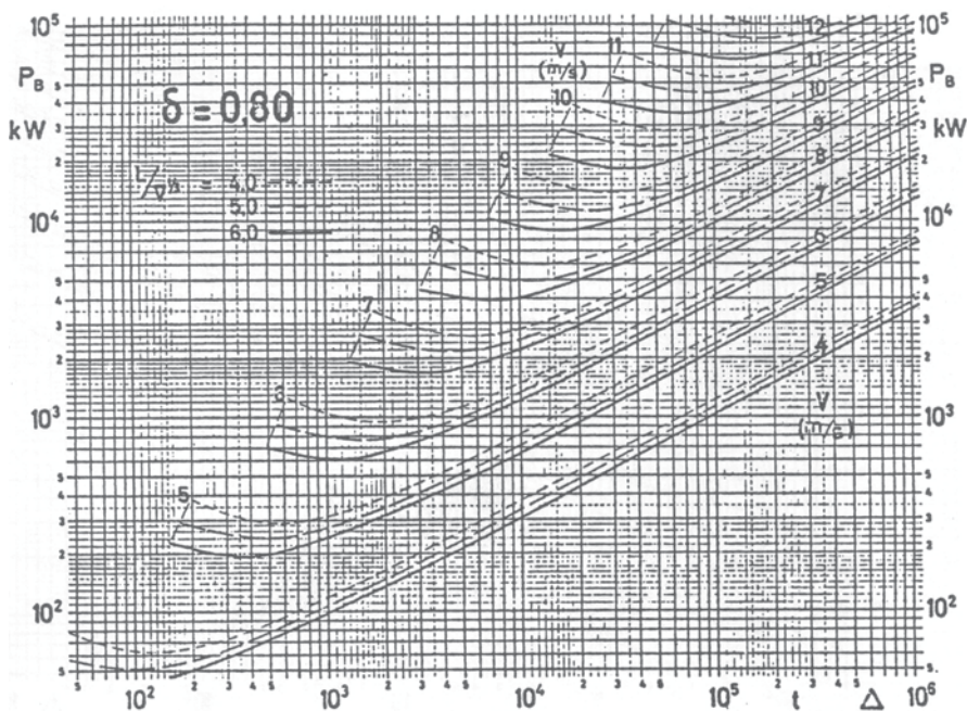
Fig. 2.65 Diagrams of installed propulsion power [kW] versus the displacement \Delta [tons], velocity V [m/s] and slenderness ratio L/V^{1/3} , C_B=0.80 acc. to Harvald
