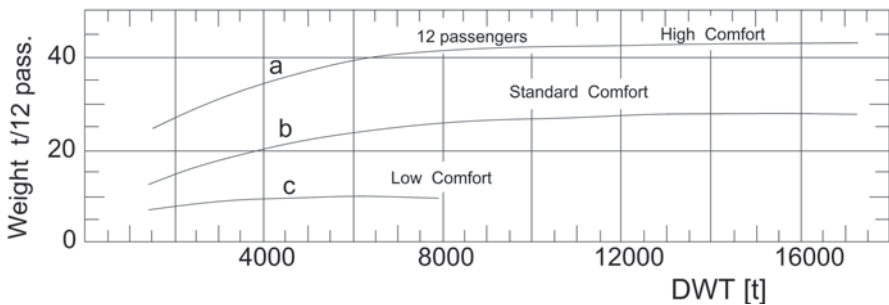
Fig. 2.81 Additional weight of accommodation outfit for 12 passengers vs. the DWT by Henschke (1964)
