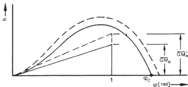
Fig. 2.36 Effect of increasing the beam on righting/restoring arm h = GZ(\varphi) : increase of value of initial stability ( GM ) and usually increase of GZ_{max} and of the range of the stability (increase of angle of vanishing stability \varphi_C )
