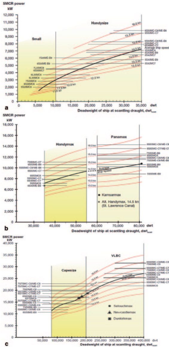
Fig. 2.62 Diagrams of installed propulsion power for Bulk Carrier versus DWT and speed V [knots]
