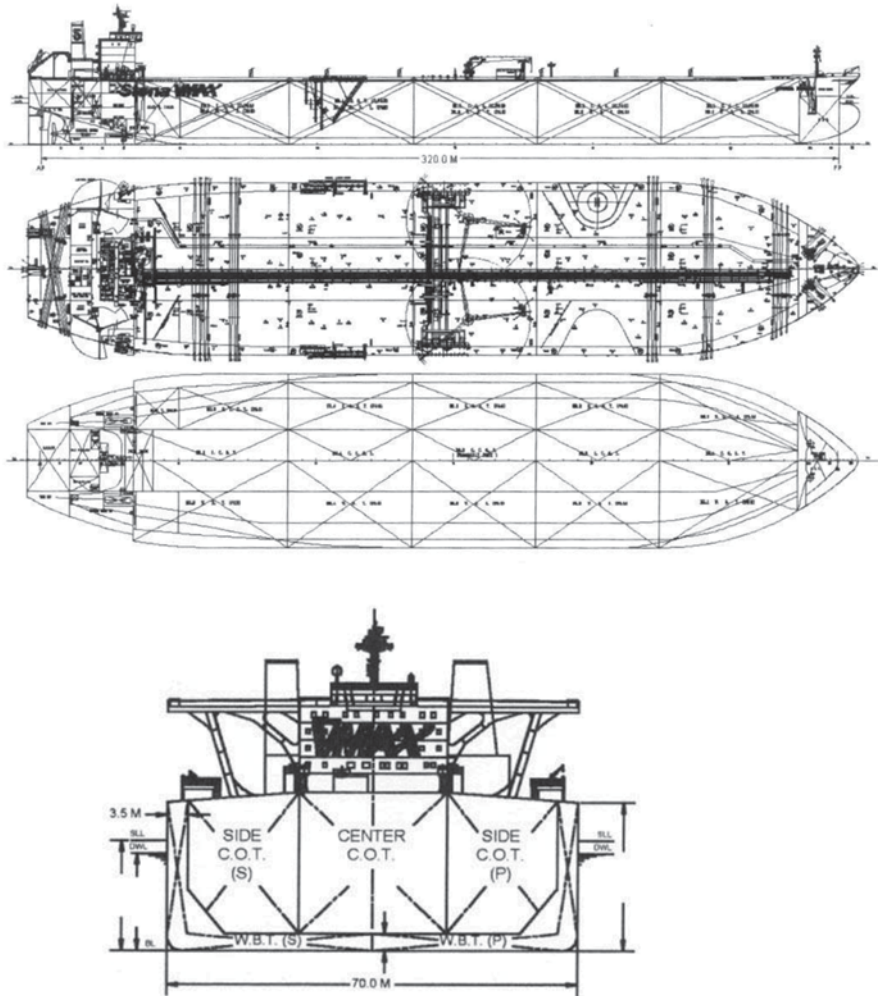
Fig. 4.16 General arrangement of a shallow draft VLCC tanker STENA VISION (Lamb 2003). (Dimensions: L_{BP}=320.0 m, B=70.0 m, T_d=16.76 m, D=25.60 m, \Delta(T_d)=311,210 t, DWT ( T_d )=268,000 t)
