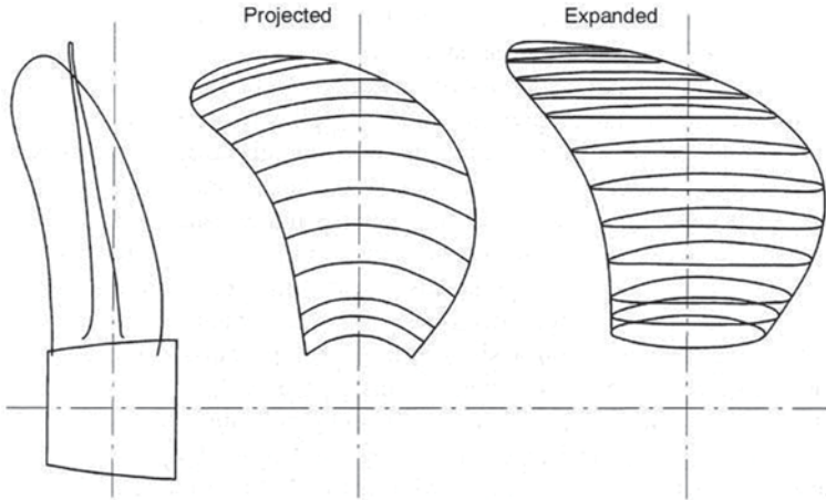
Fig. 5.15 Fixed pitch propeller geometry (Friis et al. 2002)
