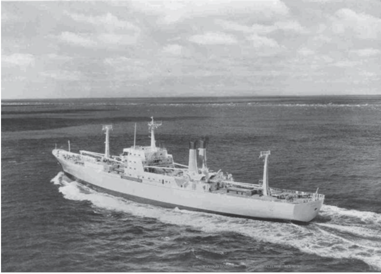
Fig. 4.12 Reefer ship “Polar Ecuador,” built in 1967 by the German yard Blohm & Voss for Hamburg Südamerikanische Dampfschiffahrts-Gesellschaft; operated later for a Greek owner as “Chios Spirit”; is representative of a successful series of fast reefer ships (service speed at banana draft: 23.5 knots) built by Blohm & Voss in the 60s, transporting bananas from South America to Europe (in German: Banana-Dampfer)
