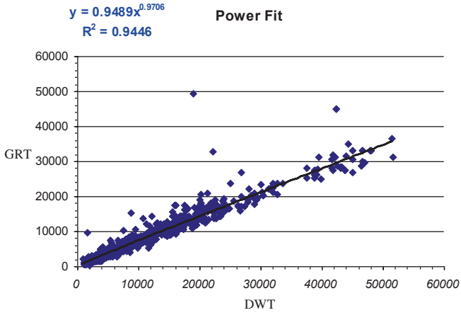
Fig. A.86 Regression analysis of GRT [RT] versus DWT [tons] for general cargo carriers (Kalokairinos et al. 2000–2005)
