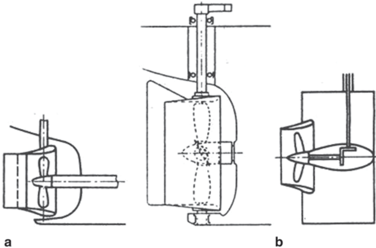
Fig. 5.39 a Kort nozzle rudder. b Pleuger active rudder
