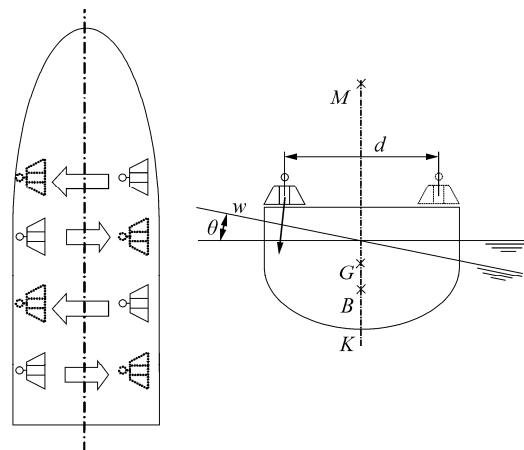
Fig. 5 Schematic diagram of the inclining experiment
