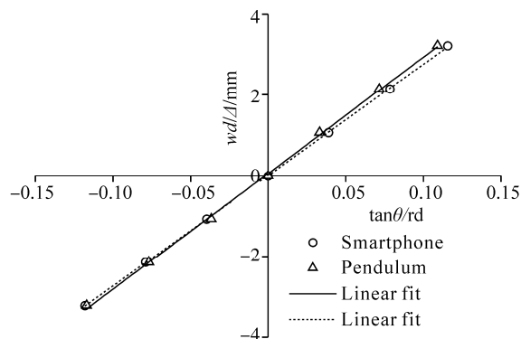
Fig. 11 wd/\Delta vs. \tan(\theta) from the inclining test
