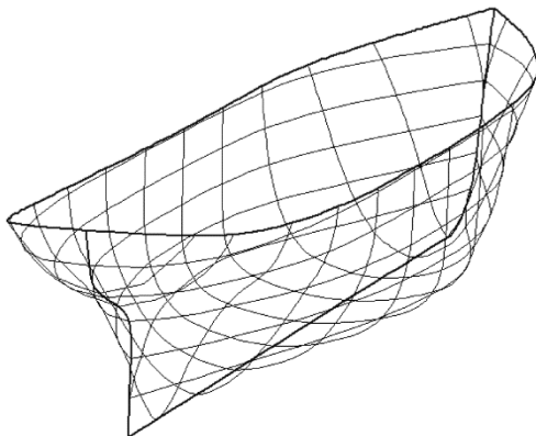
(b) Body sections and 3D view
