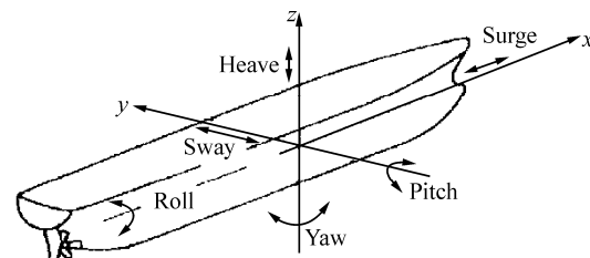
Fig. 1 Ship motions with the 6 DOF
