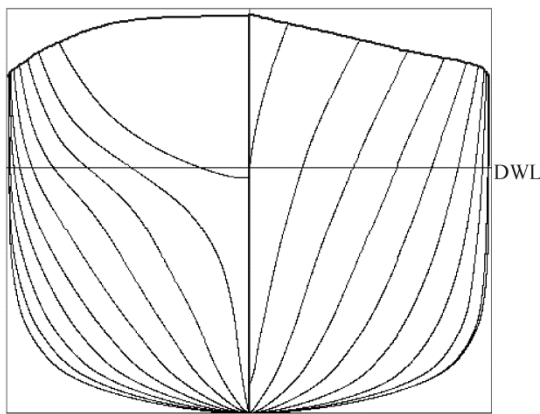
(a) Body plan
