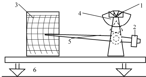
1. Knife edge; 2. Weight; 3. Rotating drum; 4. Pendulum; 5. Pen arm; 6. Adjustable table
