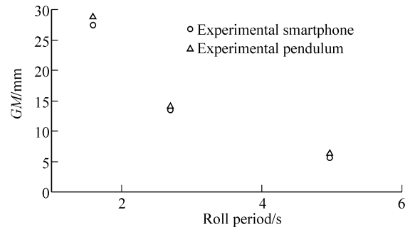
Fig. 13 Comparison of the experimental natural roll period
