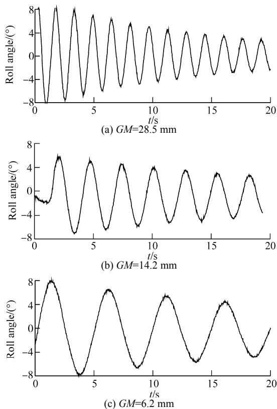
Fig. 12 Time histories data acquisition of natural rolling test for different GM
