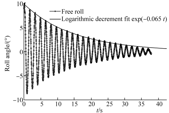
Fig. 10 Plot of the recorded CSV file of the free roll
