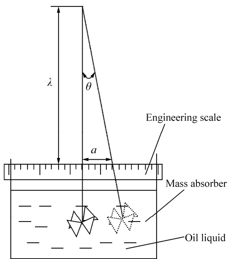
Fig. 4 Traditional tilt measurement based on a pendulum
