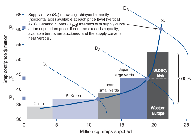
Figure 15.5 Short-run bulk shipbuilding demand and supply functions Source: Martin Stopford 2007
