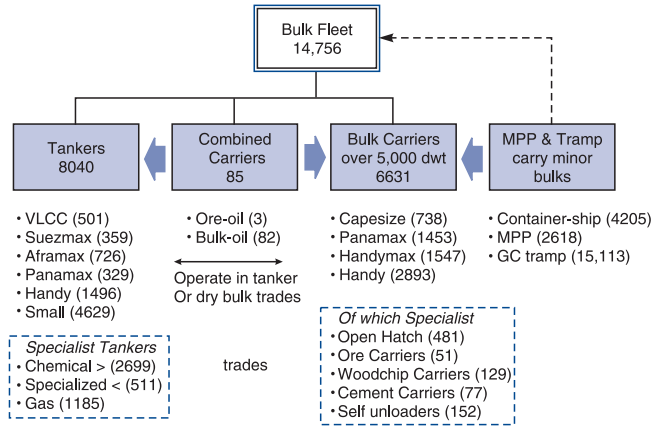
Figure 11.1 The bulk fleet showing main segments, 1 July 2007 Source: Table 2.5
