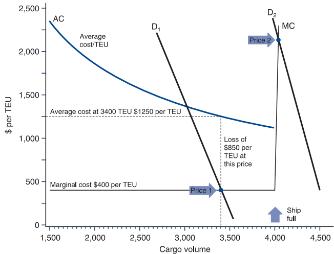
Figure 13.13 Liner pricing, Case 1: Marginal cost pricing Source: Martin Stopford, 2006
