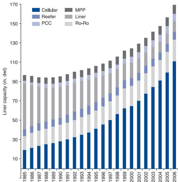
Figure 13.8 Liner fleet by vessel type, 1985–2006 Source: Clarkson Research Services Ltd
