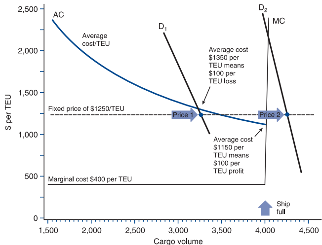
Figure 13.14 Liner pricing, Case 2: Fixed pricing Source: Martin Stopford, 2006
