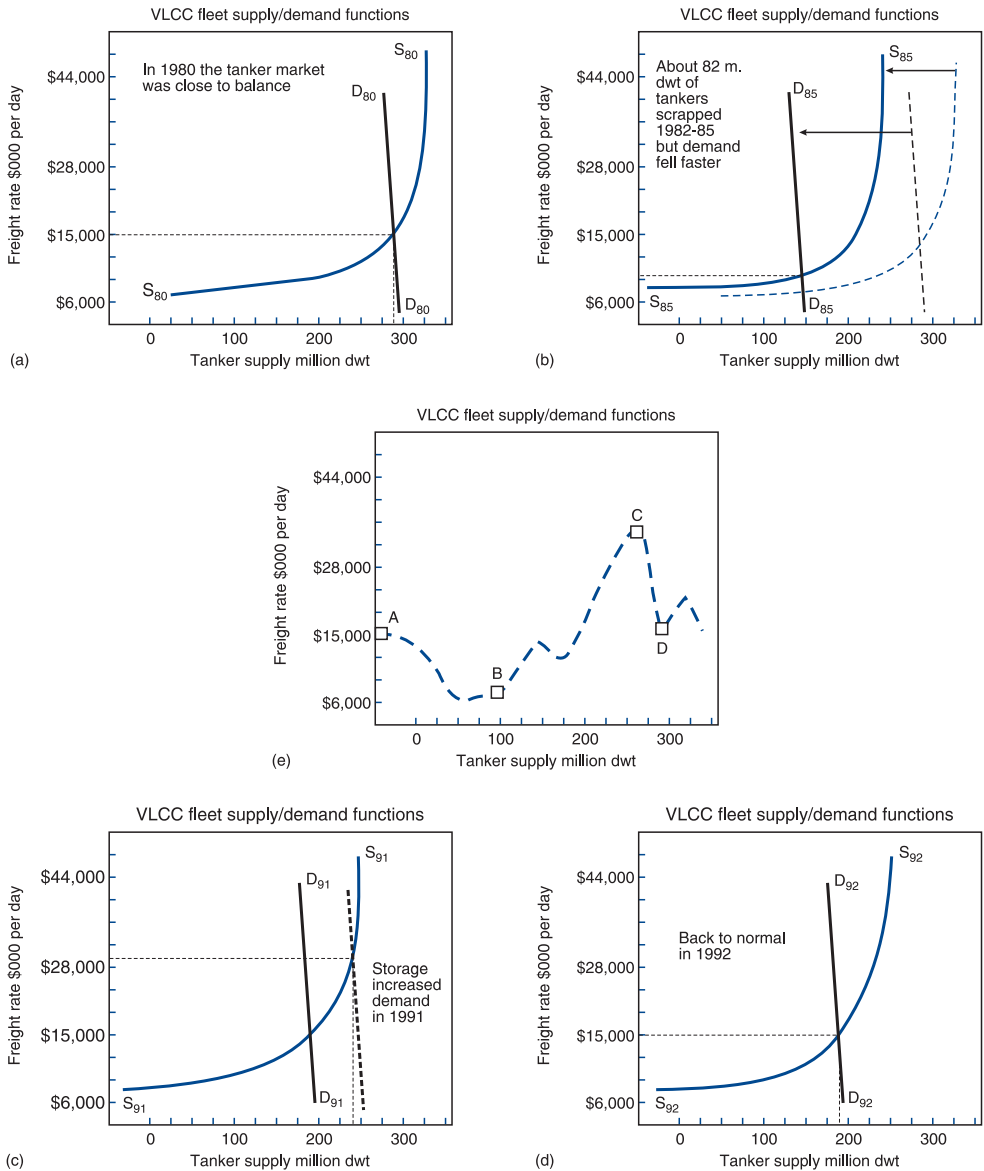
Figure 4.15 Long-term adjustment of supply and demand, 1980–92 Source: Martin Stopford 2004
