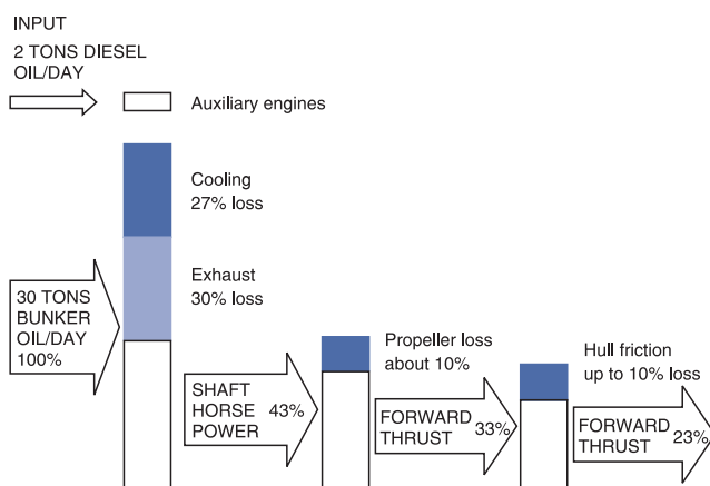
Figure 6.6 Energy losses in typical 1990s built Panamax bulk carrier, 14 knots design speed
