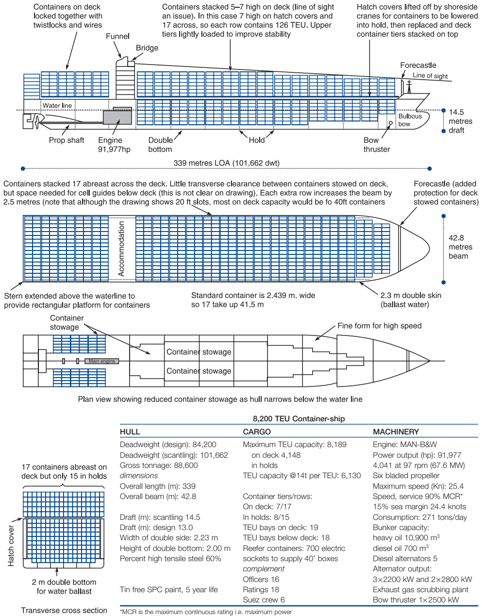
Figure 14.3 Example of typical 8,200 TEU container-ship design Source: Drawing by Martin Stopford, based on container-ships built by Hyundai Heavy Industries
