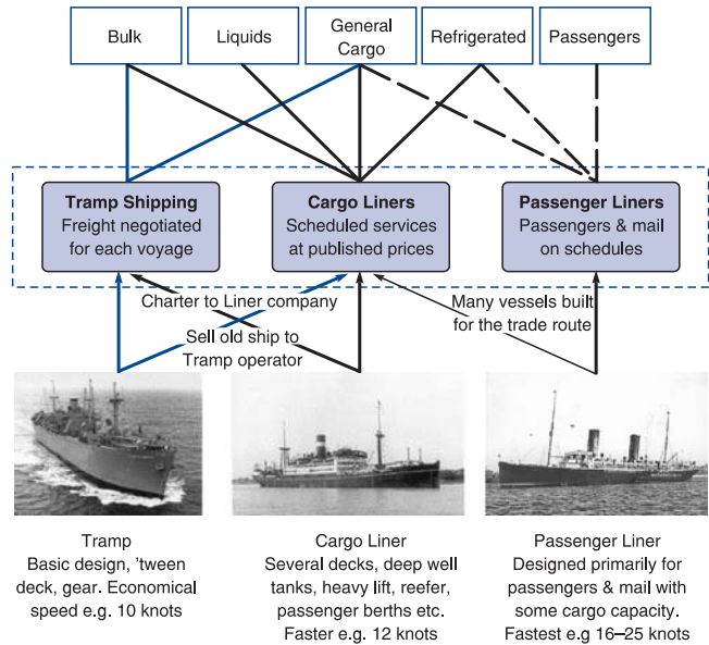
Figure 1.9 The liner and tramp shipping system, 1869–1950
