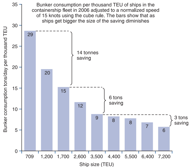
Figure 13.10 Bunker consumption of container-ships, 2006 Source: Clarkson Research Services Ltd
