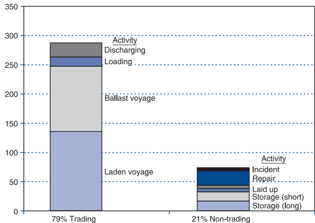
Figure 4.9 VLCC operating performance: time use of average VLCC Source: Clarkson Research Studies, VLCC Quality Survey (1991)
