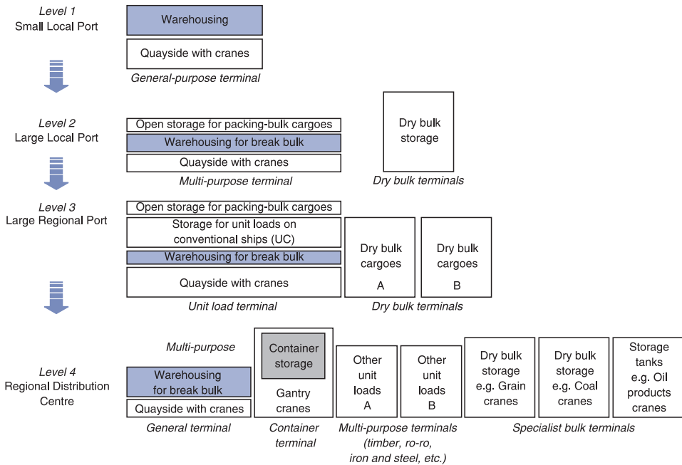
Figure 2.9 Four levels of port development Source: Compiled by Martin Stopford from various sources
