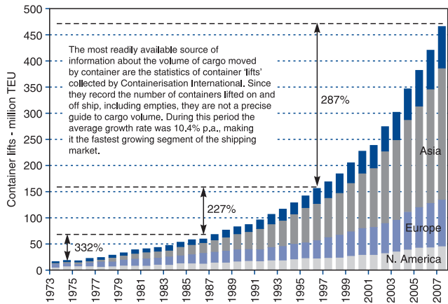
Figure 13.2 Liner trade, 1973–2007, and percentage growth per annum, 1981–2007
