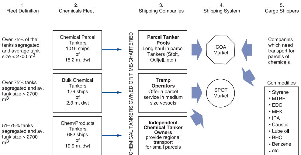
Figure 12.3 Chemical tanker sea transport system model, 2006
