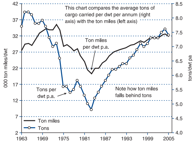
Figure 4.8 Performance of the world merchant fleet, 1963–2005 Source: Fearnleys Review
