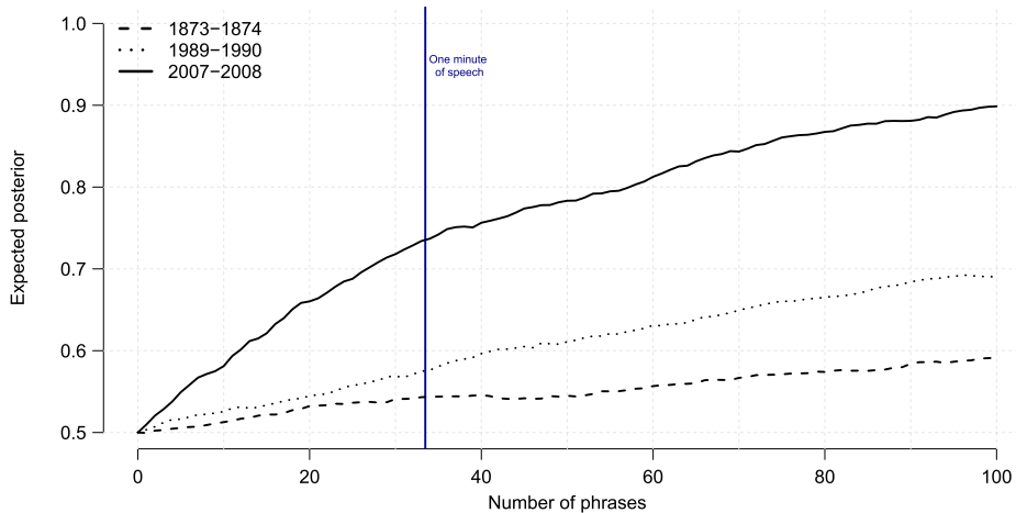
FIGURE 3.—Informativeness of speech by speech length and session. Notes: For each speaker i and session t , we calculate, given characteristics x_{it} , the expected posterior that an observer with a neutral prior would place on a speaker's true party after hearing a given number of phrases drawn according to our preferred specification in Panel B of Figure 2. We perform this calculation by Monte Carlo simulation and plot the average across speakers for each given session and length of speech. The vertical line shows the average number of phrases in one minute of speech. We calculate this by sampling 95 morning-hour debate speeches across the second session of the 111th Congress and the first session of the 114th Congress. We use https://www.c-span.org/ to calculate the time-length of each speech and to obtain the text of the Congressional Record associated with each speech, from which we obtain the count of phrases in our main vocabulary following the procedure outlined in Section 2. The vertical line shows the average ratio, across speeches, of the phrase count to the number of minutes of speech.
