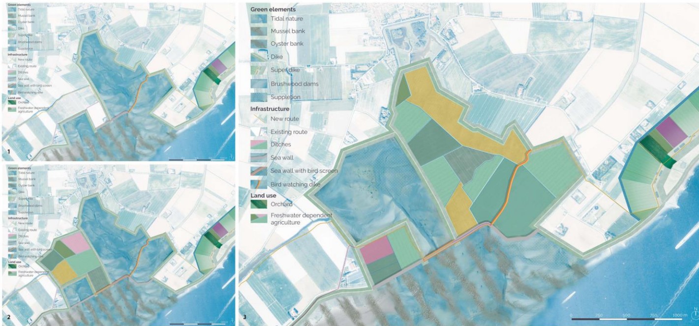
The final detailed design in three steps. A switching landscape to let problematic land silt up with SLR for nature and agriculture on the long term, with an open Oosterschelde barrier.
