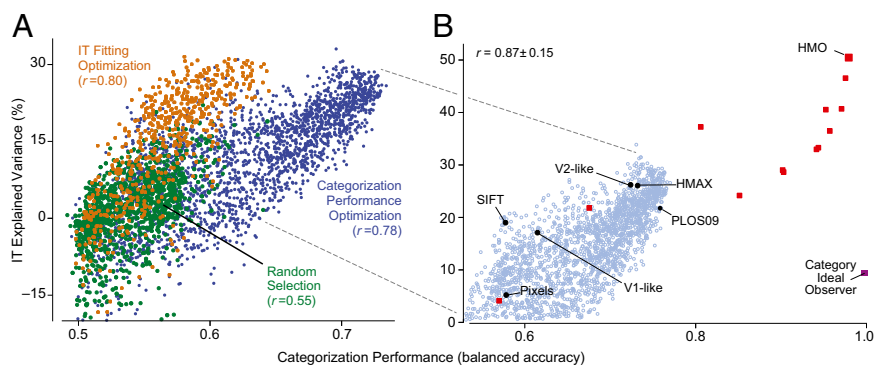
Fig. 1. Performance/IT-predictivity correlation. (A) Object categorization performance vs. IT neural explained variance percentage (IT-predictivity) for CNN models in three independent high-throughput computational experiments (each point is a distinct neural network architecture). The x axis shows performance (balanced accuracy, chance is 0.5) of the model output features on a high-variation categorization task; the y axis shows the median single site IT explained variance percentage ( n = 168 sites) of that model. Each dot corresponds to a distinct model selected from a large family of convolutional neural network architectures. Models were selected by random draws from parameter space (green dots), object categorization performance-optimization (blue dots), or explicit IT predictivity optimization (orange dots). (B) Pursuing the correlation identified in A, a high-performing neural network was identified that matches human performance on a range of recognition tasks, the HMO model. The object categorization performance vs. IT neural predictivity correlation extends across a variety of models exhibiting a wide range of performance levels. Black circles include controls and published models; red squares are models produced during the HMO optimization procedure. The category ideal observer (purple square) lies significantly off the main trend, but is not an actual image-computable model. The r value is computed over red and black points. For reference, light blue circles indicate performance optimized models (blue dots) from A.
