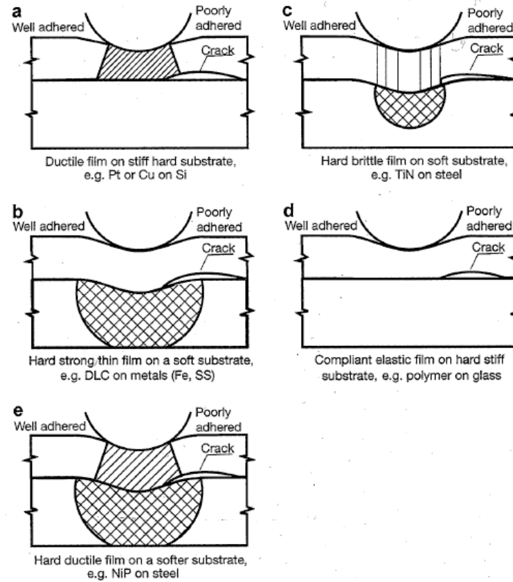
Fig. 3.62. Schematic cross-sections of various coating-substrate materials combinations and the influence of interfacial adhesion on cracking in indentation (after Swain and Mencik, 1994).
