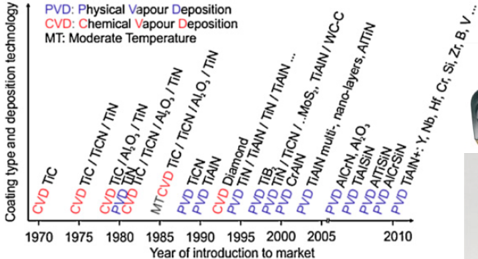
Fig. 7. Evolution of coating materials for cutting tools
