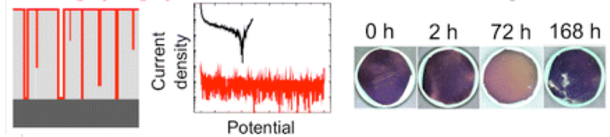
ALD \text{Al}_2\text{O}_3 - \text{Ta}_2\text{O}_5 nanolaminate sealed CrN coating on low alloy steel
