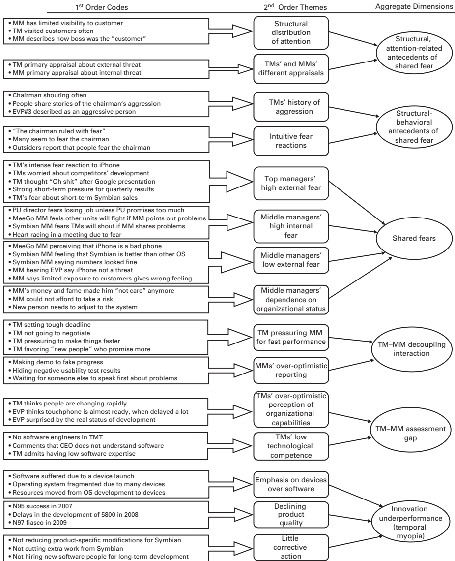
Figure 1. Code-aggregation diagram.
