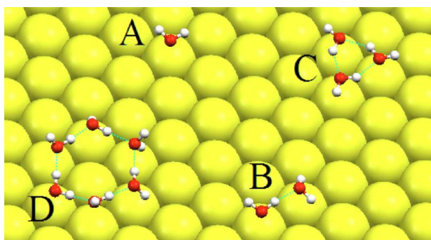
Figure: water clusters on Pt(111) surface
