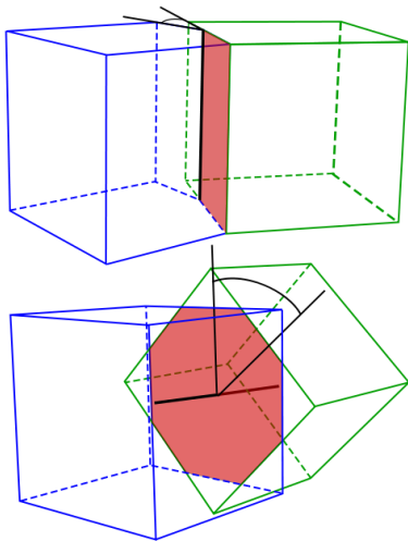
Schematic representations of a tilt boundary (top) and a twist boundary between two idealised grains.
