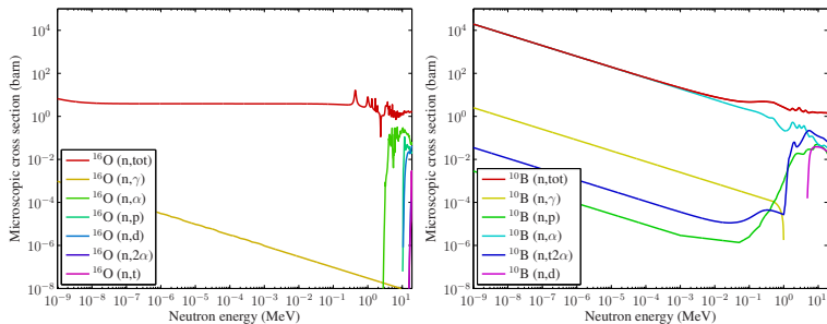
Figure 10 : Multitude of capture reactions for light nuclides. Left: The radiative capture cross section of ^{16}\text{O} is very low, and the nuclide absorbs mainly fast neutrons by (n, \alpha ). Right: ^{10}\text{B} has several capture channels available for low-energy neutrons, the most dominant of which is (n, \alpha ).
