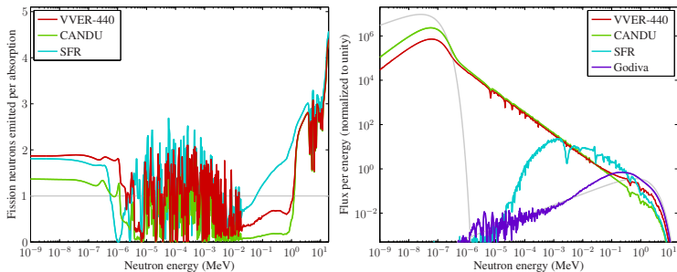
Figure 17 : Left: Average number of fission neutrons emitted per absorption to fuel as function of neutron energy in different fuel types. VVER-440 fuel is enriched to 3.6 wt-% 235 U and CANDU fuel uses natural uranium (0.72% 235 U). The sodium-cooled fast reactor (SFR) fuel is MOX, composed of depleted uranium and recycled plutonium. The fissile plutonium content is 9.6 wt-%. Right: Normalized flux spectra in the three reactor types and a fast criticality experiment (Godiva, bare HEU sphere). Shapes of the Maxwell-Boltzmann distribution at moderator temperature and the energy distribution of fission neutrons are plotted in the background. Light water reactors are typically slightly under-moderated, and the thermal peak is more pronounced in the CANDU fuel. Fast reactors operate on the other end of the flux spectrum, and lower fission cross sections are compensated by higher neutron yield and fissile mass. Even sodium has a noticeable moderating effect on neutrons, and the spectrum is clearly different from the Godiva sphere. Calculated by Monte Carlo simulation.
