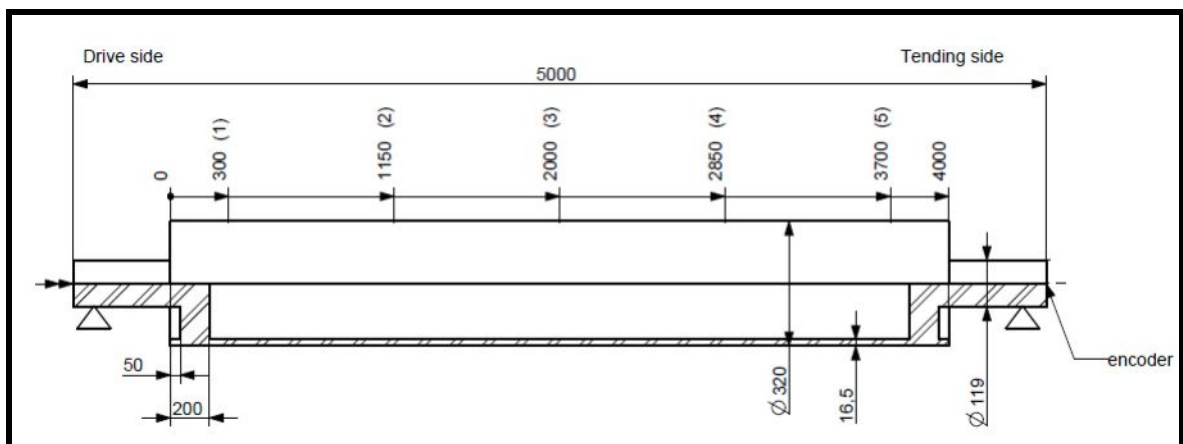
Main dimensions of the paper machine rotor (Viitala)
