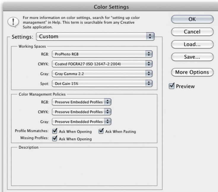
Figure 26 The Profile Mismatches settings in the Color Management section of the Color Settings dialog will influence Profile Mismatch behavior.
