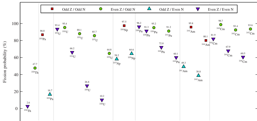
Figure 8 : Probability of fission induced by fast neutrons (Maxwellian fission spectrum peaking at 1.3 MeV). The additional kinetic energy of the neutron is sufficient to exceed the fission barrier also for most even-N nuclides.
