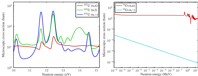
Figure 3 : Left: Elastic scattering, fission and radiative capture cross sections of ^{235}\text{U} in the low resonance range. The resonance structure depends on the energy levels of the compound nucleus formed during the interaction, which is why the cross sections share similar shape. Right: Elastic scattering and radiative capture cross sections of ^{16}\text{O} . The 1/v background shape of (n, \gamma ) cross sections is clearly seen in light nuclides without low-energy resonances. Elastic potential scattering cross section is independent of energy, and the increase at very low energy results from thermal motion.
