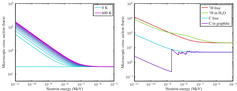
Figure 11 : Left: Effect of temperature on low-energy elastic scattering cross section of ^1\text{H} . The cross sections are plotted for 50 K intervals between 0 and 600 K. Right: Free-atom elastic scattering cross sections of ^1\text{H} and carbon compared to corresponding bound-atom cross sections in light water and graphite (all cross sections at 300 K). Neutron energies corresponding to wavelengths equal to multiples of interatomic spacing are reflected in the cross section of graphite.
