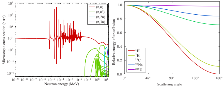
Figure 12 : Left: Elastic and inelastic scattering cross sections of ^{238}\text{U} . Right: L-frame energy transfer in elastic scattering as function of C-frame scattering angle according to Eq. (9) for target nuclides of different mass.
