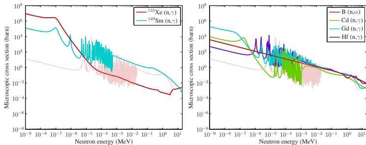
Figure 2 : Microscopic cross sections of strong absorbers. Left: Fission product poisons. Right: absorbers used for reactivity control. Capture cross section of ^{238}\text{U} is plotted in the background for comparison.
