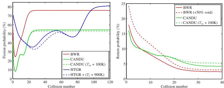
Figure 24 : Fission and return probabilities as function of collision number for different reactor types. Left: Probability of a neutron to undergo fission if its next collision occurs in fuel. The probability drops while passing through the resonances of ^{238}\text{U} , which requires different number of collisions for different moderators. The dashed blue line shows the mechanism behind the Doppler-feedback, as the fuel temperature in the HTGR case is increased from 300K to 1200K. Moderator temperature feedback is demonstrated in the CANDU case, with a temperature increase from 500K to 600K (see also Fig. 23). Right: Probability of a neutron colliding in the moderator to undergo its next collision in fuel. The dashed red line demonstrates the effect of increasing neutron mean-free-path (mfp) when the void fraction in the BWR case is increased from 25% to 75% (see also Fig. 22). Similar effect is seen for thermalized neutrons in the CANDU case, as the shift in the thermal peak increases the average mfp.
