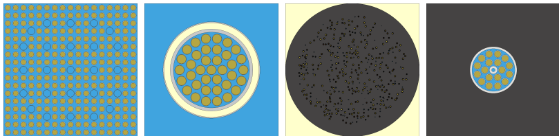
Figure 20 : Illustration of typical fuel geometries in light-water, heavy-water and graphite-moderated systems. From left to right: 1) Standard 17 \times 17 PWR fuel assembly, 2) CANDU fuel bundle inside pressure tube and moderator tank, 3) HTGR graphite pebble with 15,000 microscopic fuel particles, 4) RBMK fuel bundle inside pressure tube and graphite block. Moderator volume required to slow neutrons down to thermal region increases with nuclide mass. The fuel pins in figure 1,2 and 4 are 0.8, 1.2 and 1.2 cm in diameter, respectively. The diameter of the fuel pebble is 6.0 cm, and the coated fuel particles are less than 1 mm in size.
