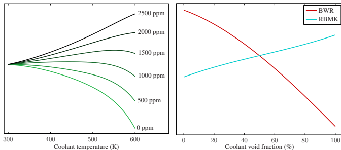
Figure 25 : Left: Effect of boron concentration in PWR coolant temperature feedback on reactivity. When the concentration of soluble absorber exceeds a certain limit, the positive reactivity from reduced absorption overwhelms the negative effect from reduced moderation as the coolant expands. Right: Negative (BWR) and positive (RBMK) reactivity feedbacks from coolant boiling. The RBMK reactor is over-moderated by graphite, and water coolant acts as a weak absorber. All calculations were carried out using Monte Carlo simulations in infinite-lattice geometries. Core-level effects and Doppler-feedback from fuel temperature are not taken into account.
