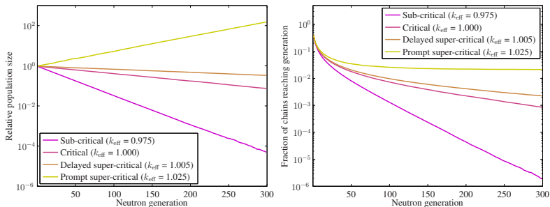
Figure 14 : Simulated prompt fission chains in a LWR fuel lattice close to criticality. Left: Relative average population size as function of neutron generation. Right: Fraction of fission chains that reach the given generation. In a critical state, more than 99% of all prompt fission chains die out during the first 100 generations. When the system reaches prompt critical state, about 2% of initiated chains continue to expand indefinitely. Calculated using Monte Carlo simulation.
