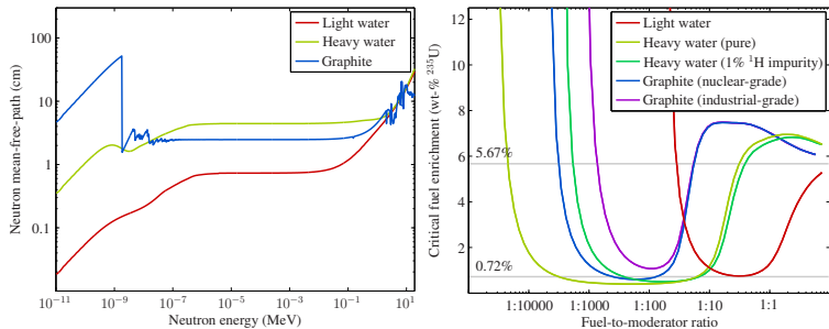
Figure 19 : Left: Neutron mean-free-path (mfp) to elastic scattering as function of energy in light and heavy water and graphite. The differences in mfp and the number of collisions required to reach the thermal region explain the differences in moderator volume for different reactor types. Right: Critical enrichments for common moderator materials as function of fuel-to-moderator ratio (FMR). Calculations are performed for a metallic 1 cm diameter uranium pin in an infinite hexagonal lattice surrounded by moderator. FMR is defined as the atomic ratio of uranium to moderator atoms ( 1 H, 2 H or 12 C). Infinite mass of uranium metal becomes critical at 5.67% enrichment without any moderation. The 235 U content in natural uranium is 0.72%. Nuclear- and industrial-grade graphite refer to boron impurities of 1 and 20 ppm, respectively.
