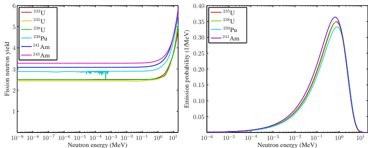
Figure 5 : Left: Fission neutron yields of various actinides as function of neutron energy. The yield is actually a linear function of energy, which only appears to increase sharply in the MeV-range because of the logarithmic scale. The number of emitted neutrons increases along with actinide mass. Right: The Maxwellian energy distributions of ^{235}\text{U} , ^{238}\text{U} , ^{239}\text{Pu} and ^{241}\text{Am} fission neutrons. The peak position varies slightly for different actinides, but is practically independent of neutron energy. The average energy for ^{235}\text{U} fission neutrons is around 2 MeV.
