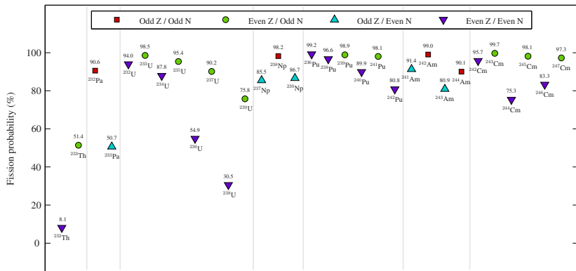
Figure 9 : Probability of fission induced by high-energy neutrons (14 MeV). Fission probability becomes even higher when the energy exceeds 10 MeV, but these energies are not very relevant for conventional fission applications.
