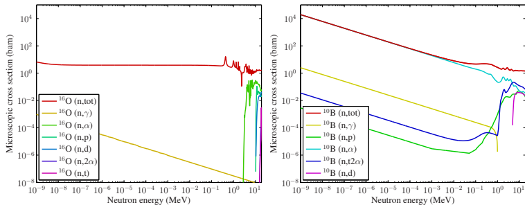
Figure 10 : Multitude of capture reactions for light nuclides. Left: The radiative capture cross section of 16 O is very low, and the nuclide absorbs mainly fast neutrons by (n,α). Right: 10 B has several capture channels available for low-energy neutrons, the most dominant of which is (n,α).
