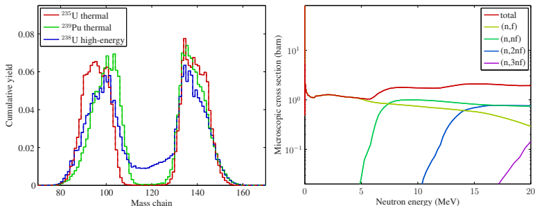
Figure 4 : Left: The double-peaked fission product distribution. The yields are calculated as cumulative values over each mass chain. The lower peak shifts to the right as the mass of the fissioned actinide increases. High-energy fission for ^{238}\text{U} refers to reaction caused by 14 MeV neutrons. Increasing neutron energy lifts the distribution between the two peaks. Right: Total fission cross section of ^{235}\text{U} divided into 1st-, 2nd-, 3rd-, and 4th-chance fission components. The higher modes are threshold reactions that increase the total cross section in the MeV-range.
