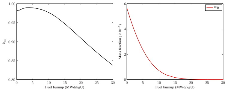
Figure 27 : Depletion of a “gray” boron silicate glass burnable absorber in a PWR fuel assembly calculation. Left: Infinite multiplication factor, Right: Absorber concentration. The absorber is natural boron (20% ^{10}\text{B} , 80% ^{11}\text{B} ), but only the high-absorbing isotope is depleted.
