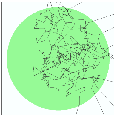
Figure 13 : Neutron tracks of a prompt fission chain initiated by a single neutron introduced into a critical system. Infinite uranium cylinder with 6.2 cm diameter and 10% ^{235}\text{U} enrichment. The initiating neutron produces 43 descendants and the chain dies out in 0.55 \mu\text{s} . The tracks are animated in Lecture1_anim1.gif . For similar animation of a prompt super-critical system, see Lecture1_anim2.gif .
